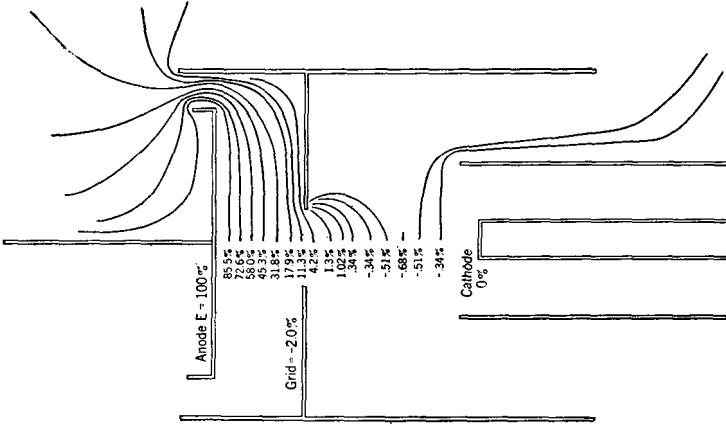
By permission of the publishers of Electronica . Fig. 58. Potential distribution in a "negative-grid" tube at breakdown.
