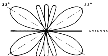
2\frac{1}{2} WAVE ANTENNA (5TH HARMONIC)
