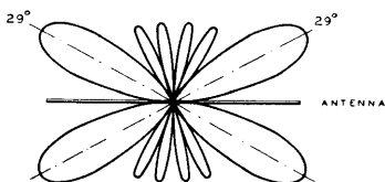
3 WAVE ANTENNA (6TH HARMONIC)
