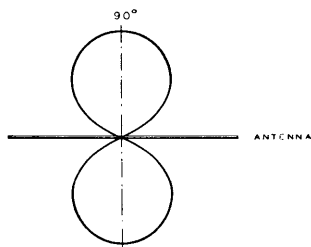
HALF WAVE ANTENNA (1ST HARMONIC OR FUNDAMENTAL)
