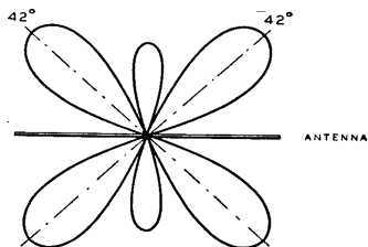
1\frac{1}{2} WAVE ANTENNA (3RD HARMONIC)
