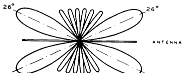
4 WAVE ANTENNA (8TH HARMONIC)
