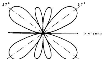
2 WAVE ANTENNA (4TH HARMONIC)
