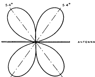
FULL WAVE ANTENNA (2ND HARMONIC)
