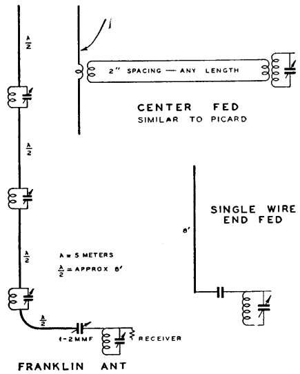
Group of Typical 5-Meter Antennas.
