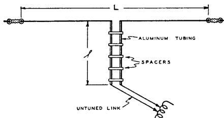
JOHNSON "Q" ANTENNA
