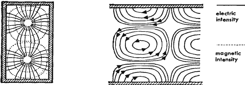
Fig. 7—Instantaneous field configuration for a TM_{1,2} wave.
