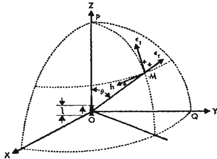
Fig. 1 Electric and magnetic components in spherical coordinates for elec- tric dipoles.
