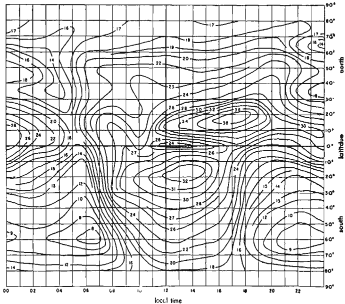
Fig. 10— F_2 4000-kilometer maximum usable frequency in megacycles. 1 zone (see Fig. 8) predicted for July, 1946.
