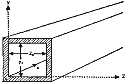
Fig. 1—Rectangular wave guide.
