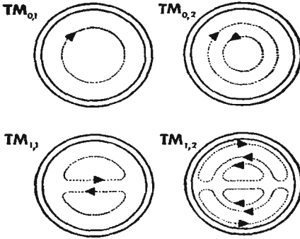
Fig. 9 Patterns of magnetic force of TM waves in circular wave guides.
