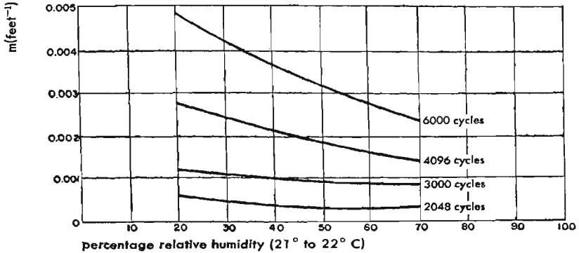
Fig. 5—Value of attenuation constant m at different frequencies and relative humidities.*
