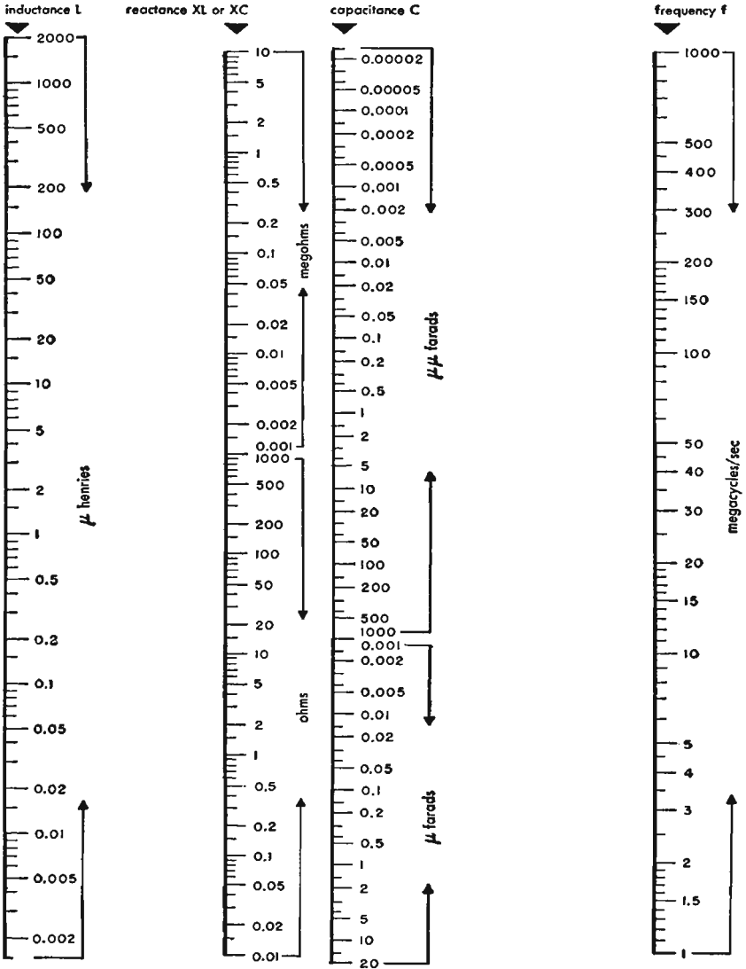
Fig. 4-1 1 megacycle to 1000 megacycles.
