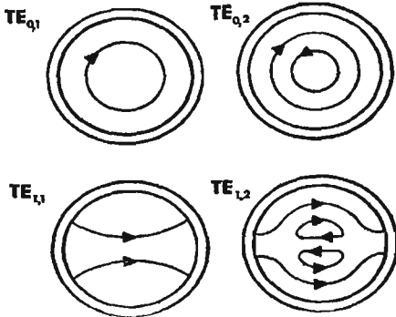
Fig. 11 Patterns of electric force of TE waves in circular wave guides.
