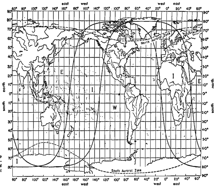
Fig. 8—World map showing zones covered by predicted chords and auroral zones.
