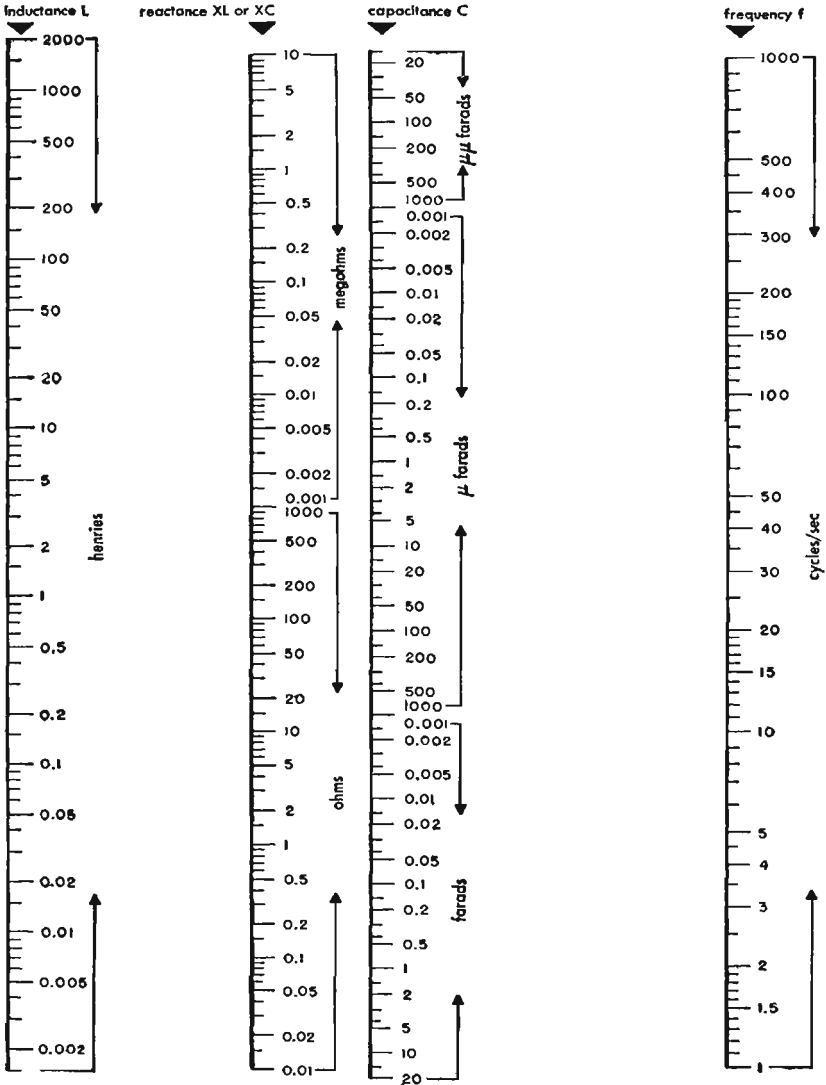
Figs 2, 3, and 4 give the relationships of capacitance, inductance, reactance, and frequency. Any one value may be determined in terms of two others by use of a straight edge laid across the correct chart for the frequency under consideration.
