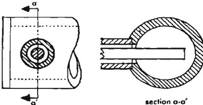
Fig. 12 Method of coupling to circular wave guide for TE_{1,1} wave.
