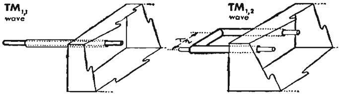
Fig. 8—Methods of coupling to rectangular wave guides for TM(E) modes.
