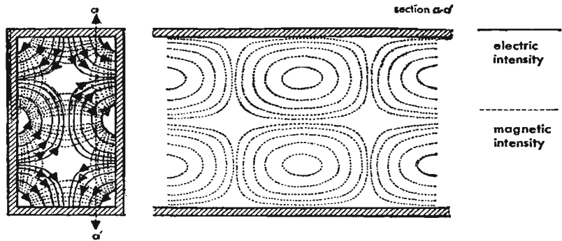
Fig. 3—Field configuration for a TE_{1,2} wave.
