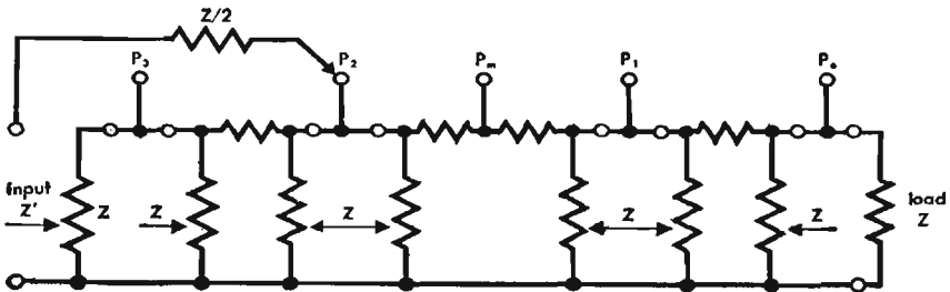
Fig. 17 —A variation of the ladder attenuator, useful when Z_1 = Z_2 = Z . Simpler in design, with improved impedance characteristics, but having minimum insertion loss 2.5 db higher than attenuator of Fig. 16. All \pi sections are symmetrical.
