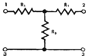
equivalent symmetrical T section
