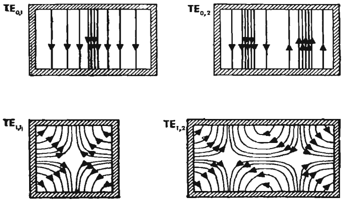
Fig. 4—Characteristic E lines for TE waves.
