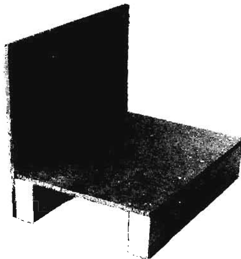
Fig. 49—Hardware cloth cut with metal shears and shaped to form a chassis. Corners are held together by soldering or by wrapping ends of wire mesh together.
