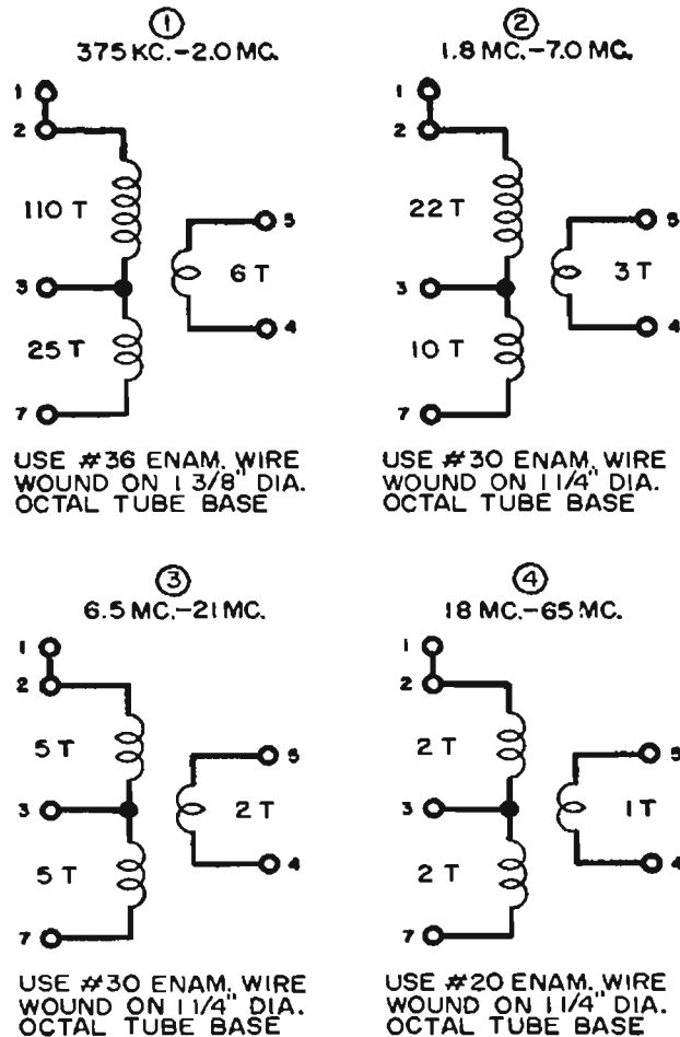
Fig. 131—Four coils required for basic frequency ranges. Use data given here to wind coils.
