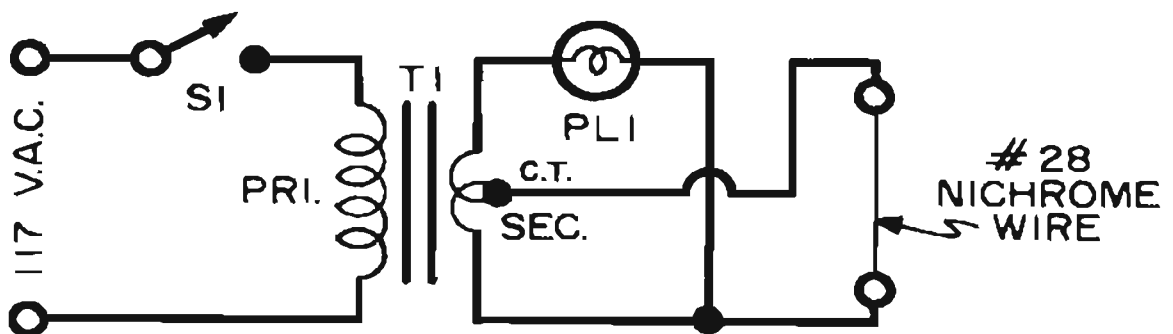
Fig. 99—Simple electrical circuit for plastic cutter heats No. 28 Nichrome wire.
