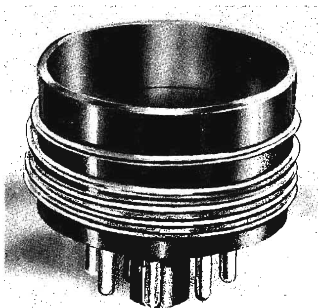
Fig. 132—Coil wound on salvaged octal tube base.
