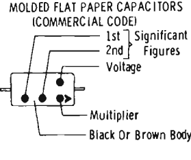
Fig. 33—Capacitor color code (continued).
