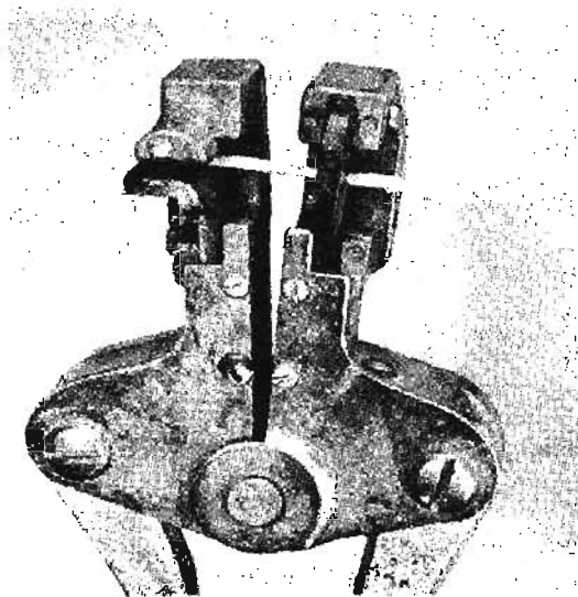
Fig. 14—Wire strippers remove insulating up to the desired point with one squeeze of the handles.
