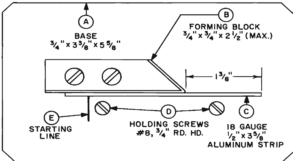
Fig. 107—Job layout. Letters refer to parts as explained in text.
