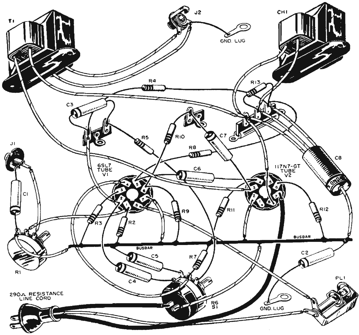
Fig. 159—Wiring of amplifier.
