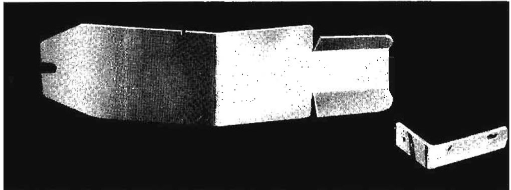
Fig. 74—Rocker fashioned from aluminum. Notches must fit snugly into narrower part of rocker cutout in aluminum mounting frame. The leaf spring is stainless steel strap and the switch bracket is aluminum.
