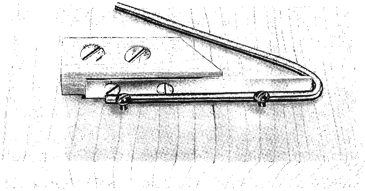
Fig. 108—Second step in making a tip for the soldering gun is to bend the 7 \frac{1}{4} -inch strip of wire back over the metal forming piece.
