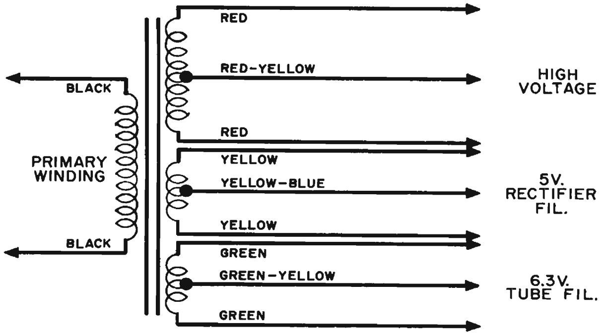
Fig. 38—Wire color coding for typical power transformer.
