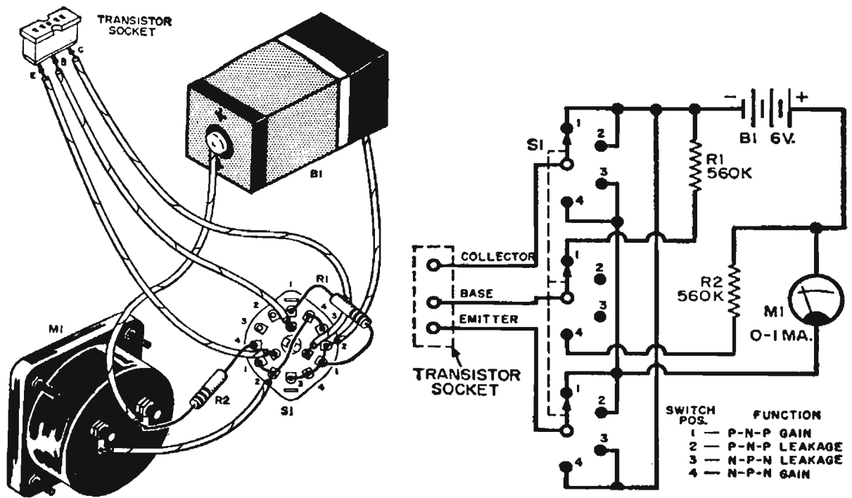
Fig. 120—Pictorial and schematic diagrams show how parts are interconnected.
