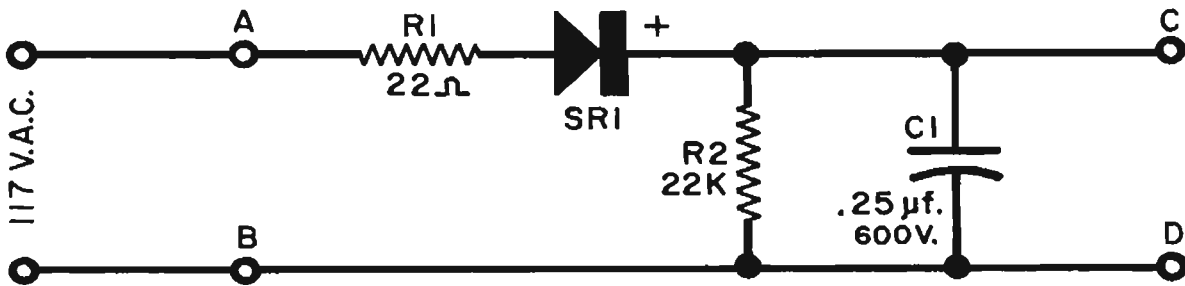
Fig. 118—Circuit layout of voltage calibrator.
