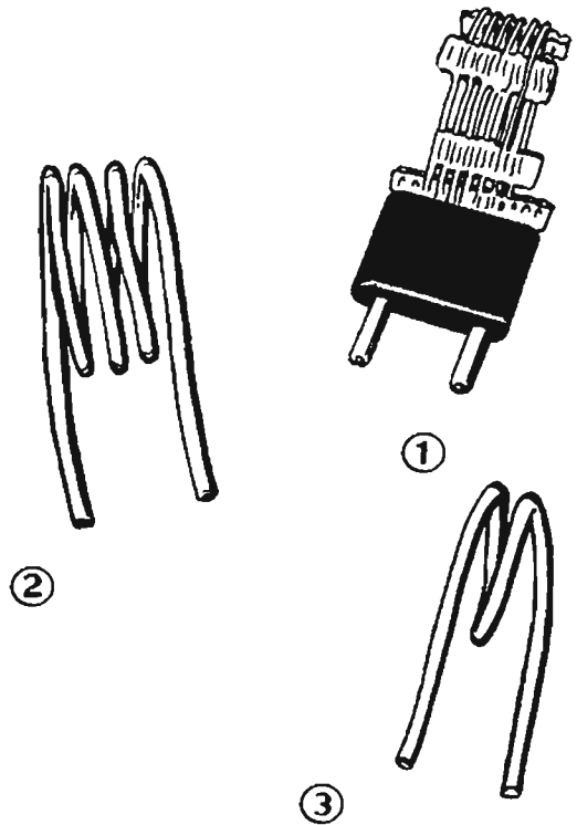
Fig. 146 (1)—For the 28-50-mc band: six turns of Barker & Williamson Miniductor No. 3015 coil stock (16 turns/inch), soldered into Millen No. 37412 plug. (2)—For the 48 to 90-mc band: four turns of No. 12 wire, tinned, \frac{1}{2} " long, 1" in diameter. (3)—For the 90-175-mc band: two turns of No. 12 wire, tinned, \frac{1}{2} " long, \frac{3}{4} " in diameter.
