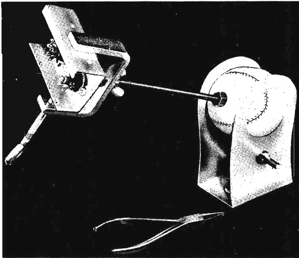
Fig. 84—Universal arm for small assemblies uses ball as movable joint.
