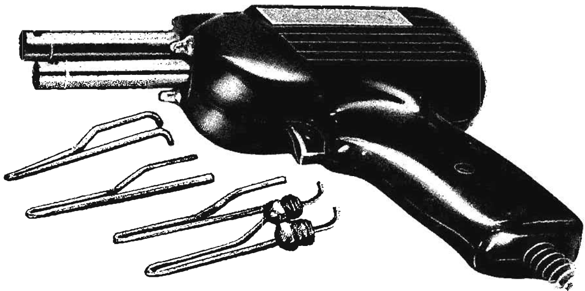
Fig. 109—Soldering gun with new tips ready for assembly. End of tips that fit into gun barrels must be bent slightly after the clamping nuts are attached.
