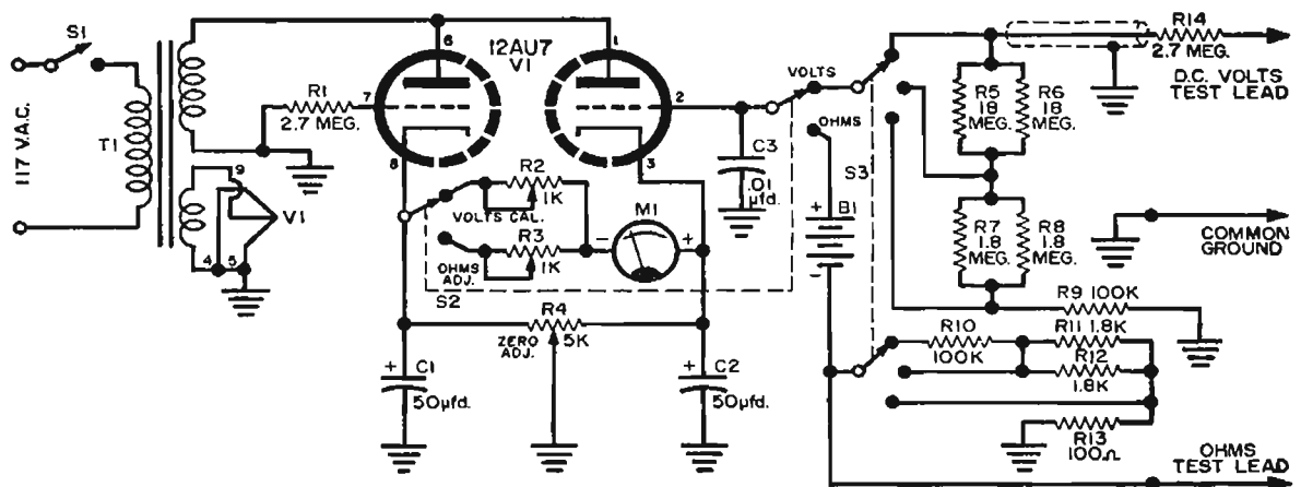
Fig. 115—Wiring diagram of test instrument. Note absence of rectifier which is found unnecessary in this circuit.
