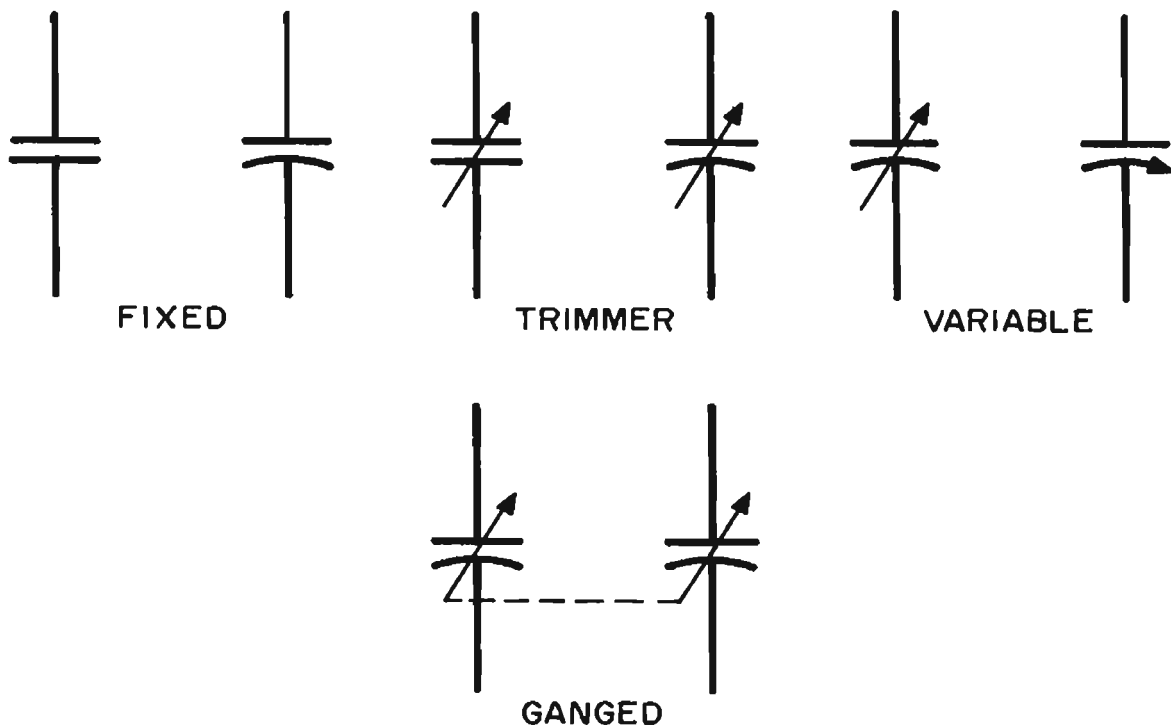
Fig. 35—Symbols for capacitors
