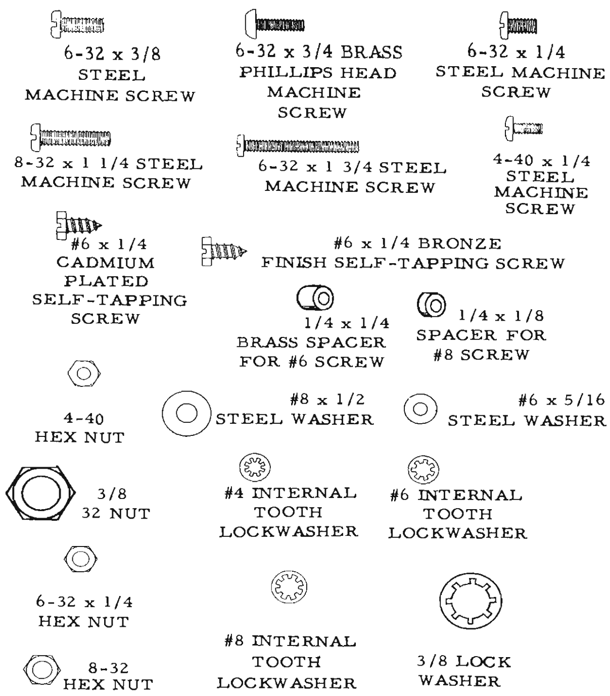
Fig. 18—Common pieces of hardware used to assemble electronic equipment.
