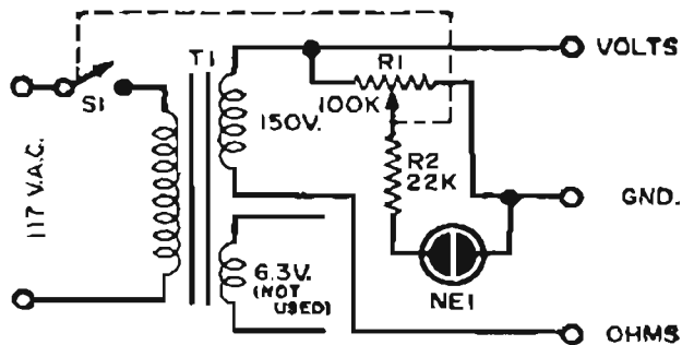
Fig. 111—Schematic diagram of multi-tester unit.
