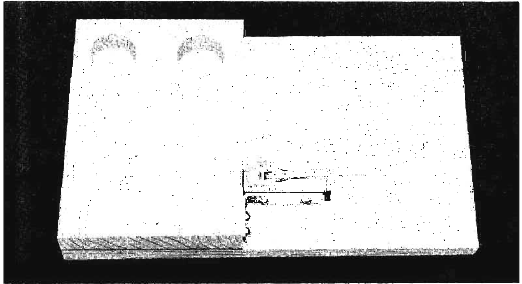
Fig. 73—Base block glued to main base. The two holes are 1\frac{1}{4} inches in diameter and must line up with holes in aluminum plate. Lever switch and bracket nestle in cutout made in main base and are secured in place with wood screws.
