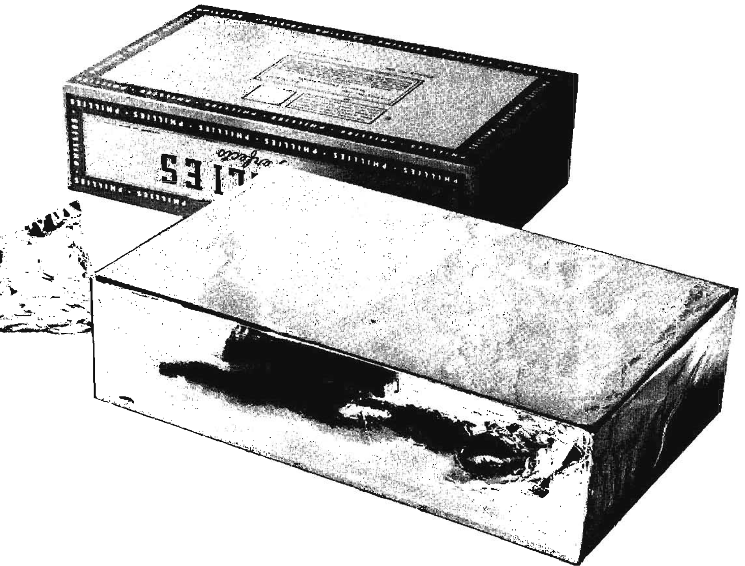
Fig. 53—A cigar box covered with aluminum foil makes a good shielded chassis.
