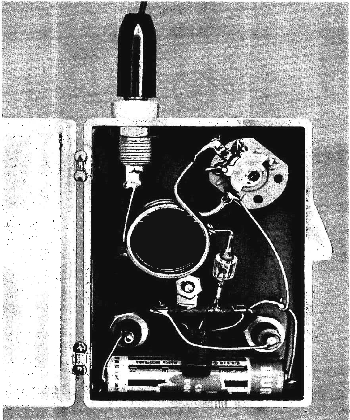
Fig. 155—Parts placement can be seen from inside photo of finished unit.
