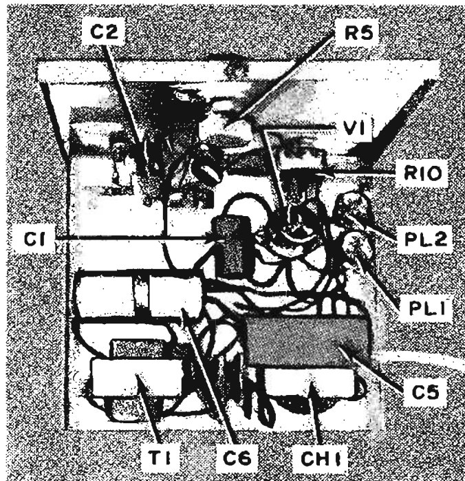
Fig. 158—Underside of amplifier chassis showing terminal board and point-to-point wiring. Note that the major components are crowded to the back of the chassis to keep hum away from the tone and volume controls.
