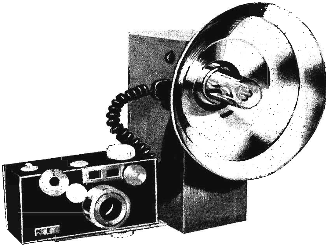
Fig. 165—Electronic photoflash uses transistor oscillator to supply high voltage for flashbulb.
