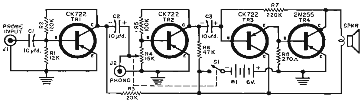
Fig. 135—Circuit of signal tracer uses three CK722's and one 2N255.
