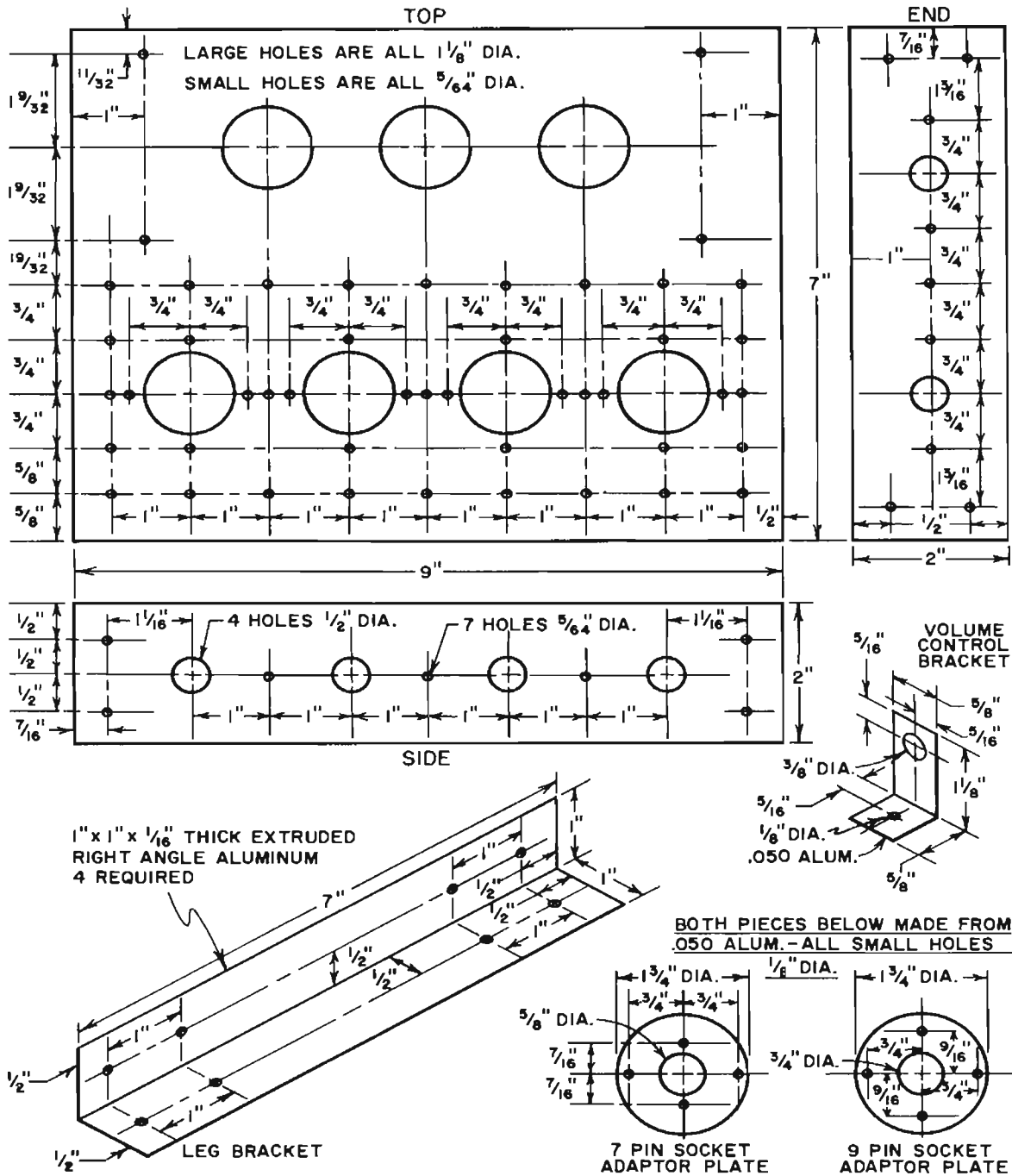
Fig. 106—Plans for assembly of permanent breadboard.
