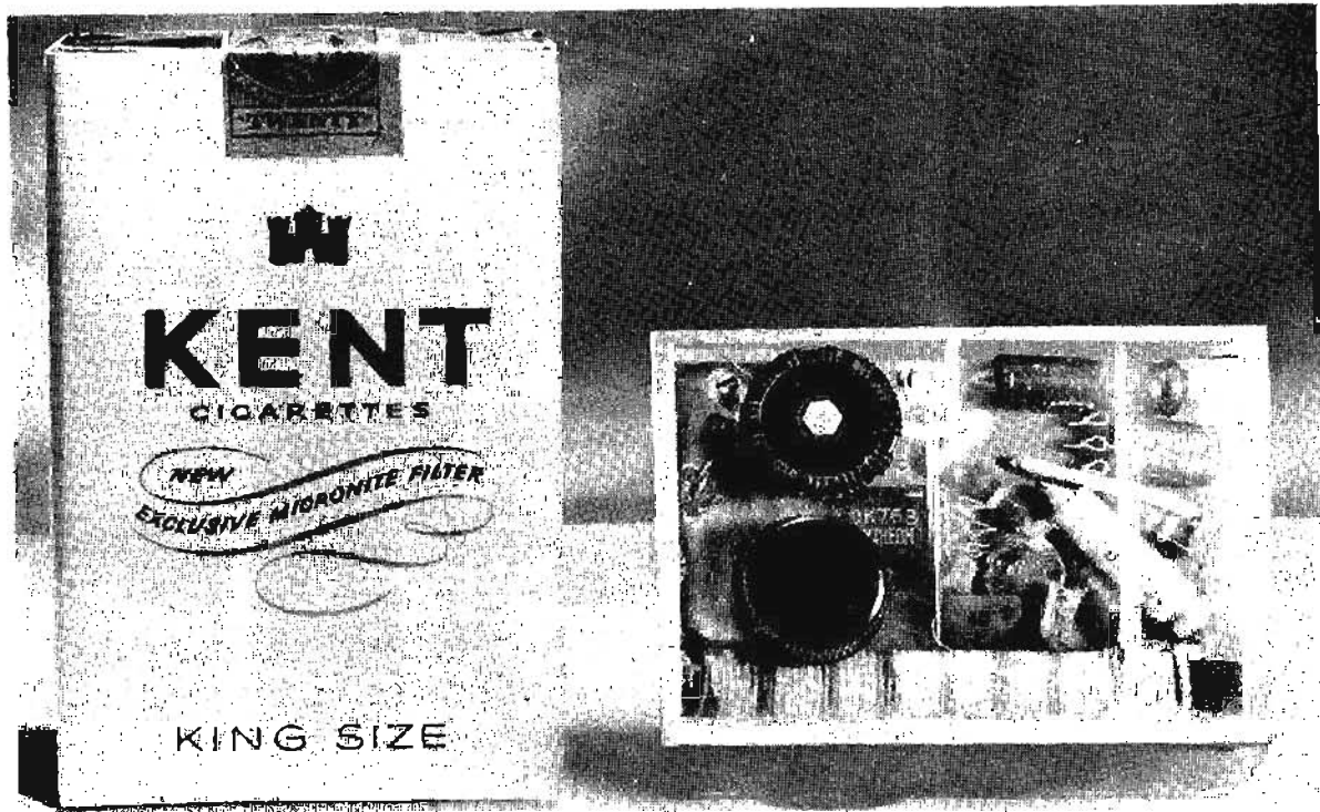
Fig. 14B—Complete transistorized receiver.
