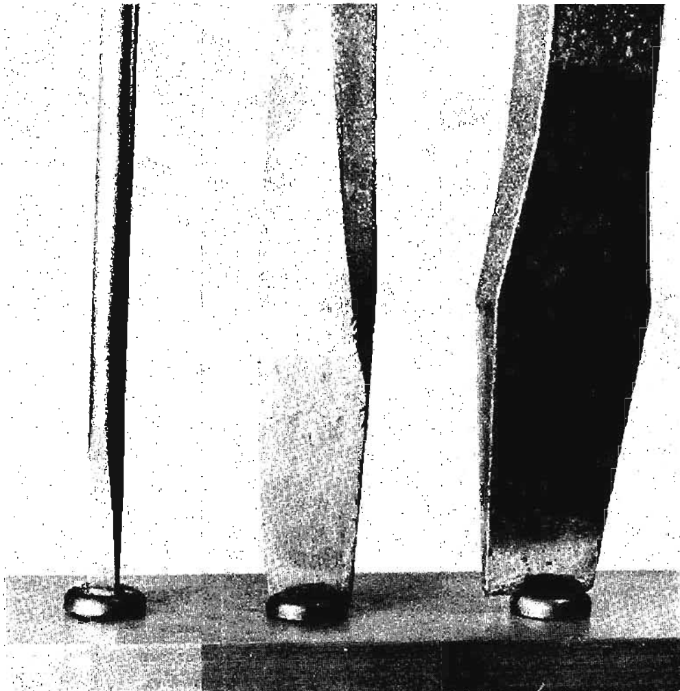
Fig. 7—The screwdriver at the left is too small; its blade could snap. Screwdriver at right is too large and could damage screw. Screwdriver in center fits snugly into slot and has proper width.
