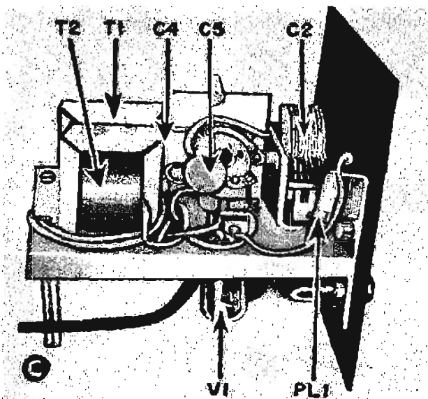
Fig 128 (2)—Three views of the signal generator chassis showing placement of major components: (A) bottom view; (B) right side view; and (C) left side view. Layout is critical.
