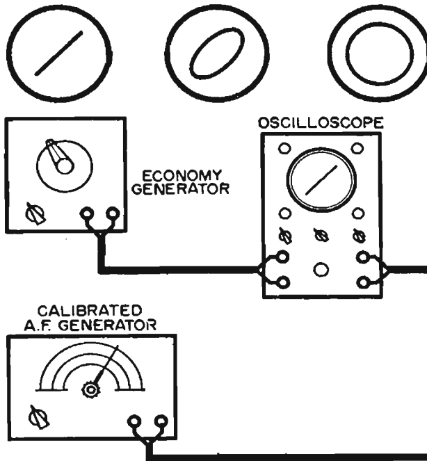
Fig. 128 (1)—Two possible methods of calibrating the audio generator.
