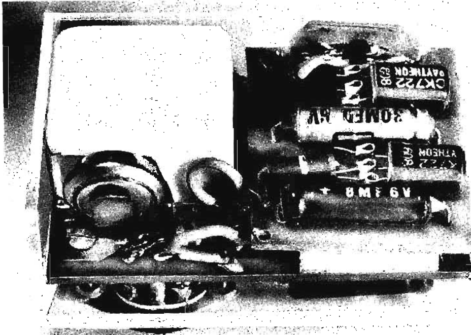
Fig. 151—Chassis with two sides installed. Tuning capacitor and battery are at left.
