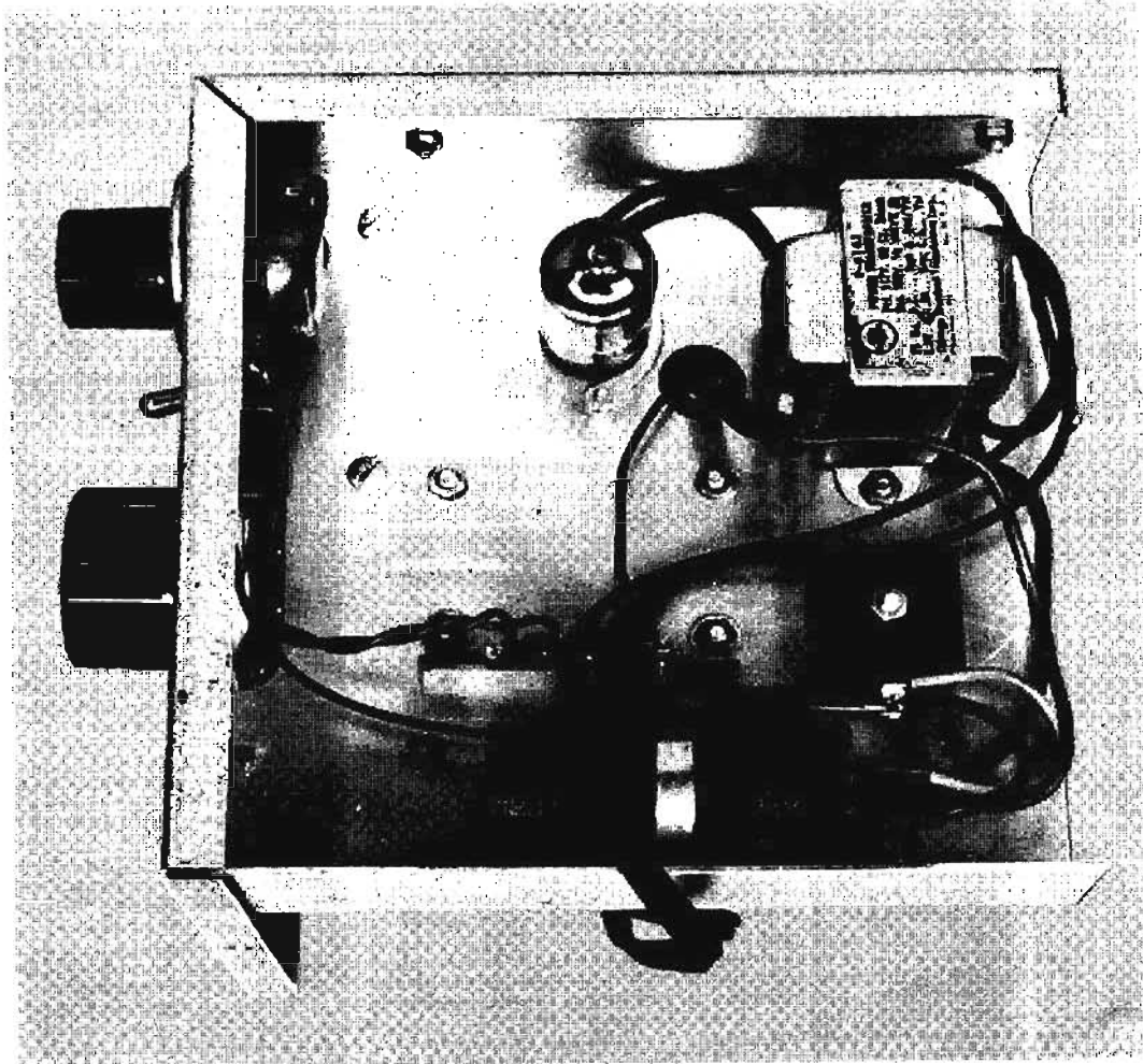
Fig. 145—Right side of receiver contains oscillator tube and coil socket into which band coils are plugged. Point-to-point wiring and short leads are used.
