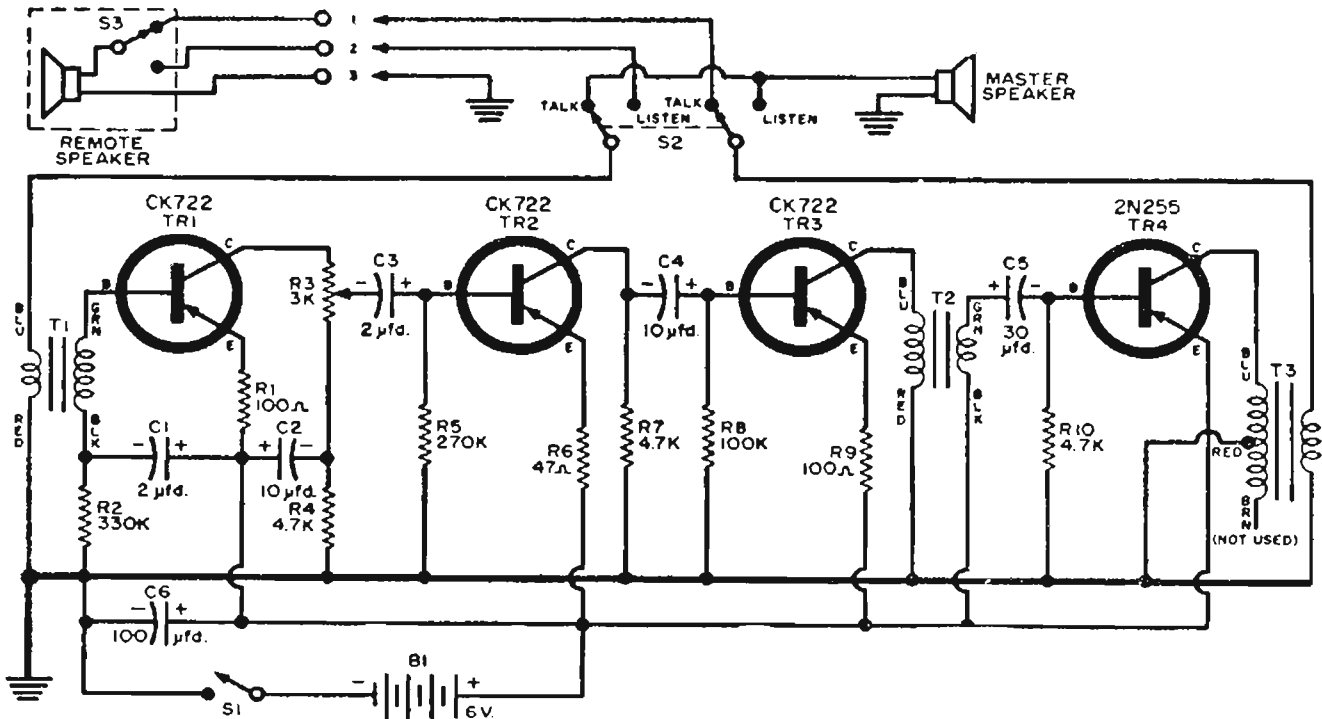
Fig. 161—Intercom circuit uses three CK722 transistors and one 2N255 power transistors.
