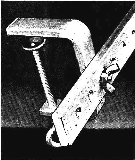
Fig. 93—Detail view of the mounting for one of the "Handy Clamps," which are manufactured by Stanley and are available from most hardware stores. To compensate for varying chassis weights, the clamps may be moved along the rocker bar to new pre-drilled positions.
