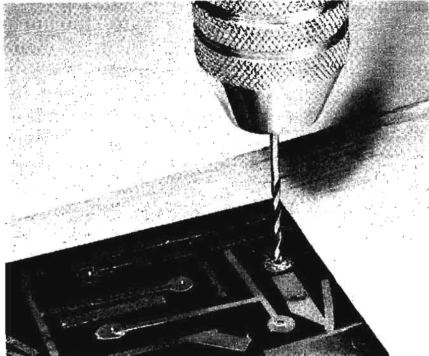
Fig. 62—Drilling component mounting holes in printed-circuit board.
