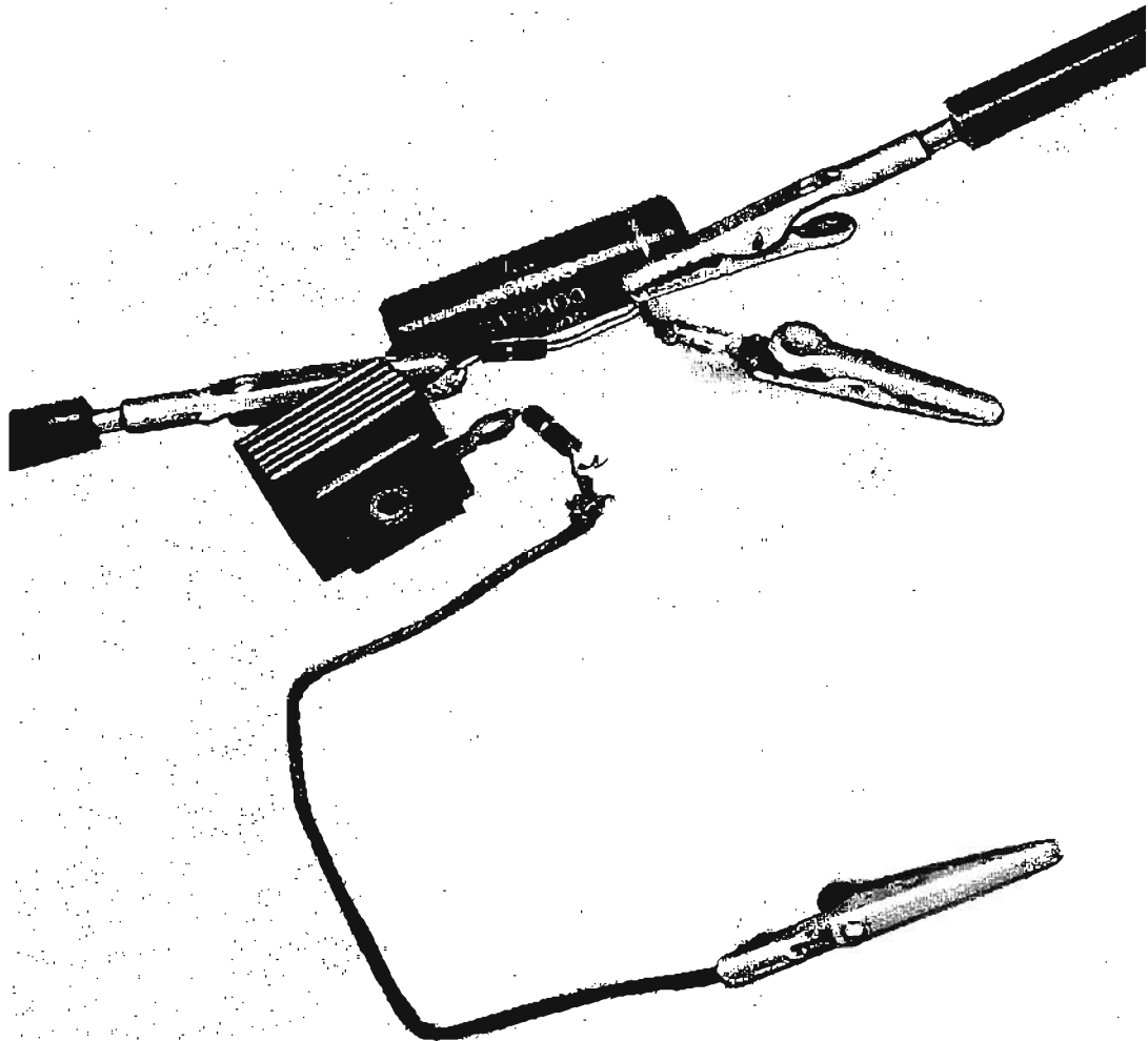
Fig. 117—Circuit of voltage calibrator is so simple that a chassis is not necessary.
