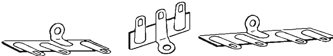
Fig. 17—Terminal strips are available in many different configurations. The center strip has one lug connected to mounting bracket so that it can be used as a chassis ground.
