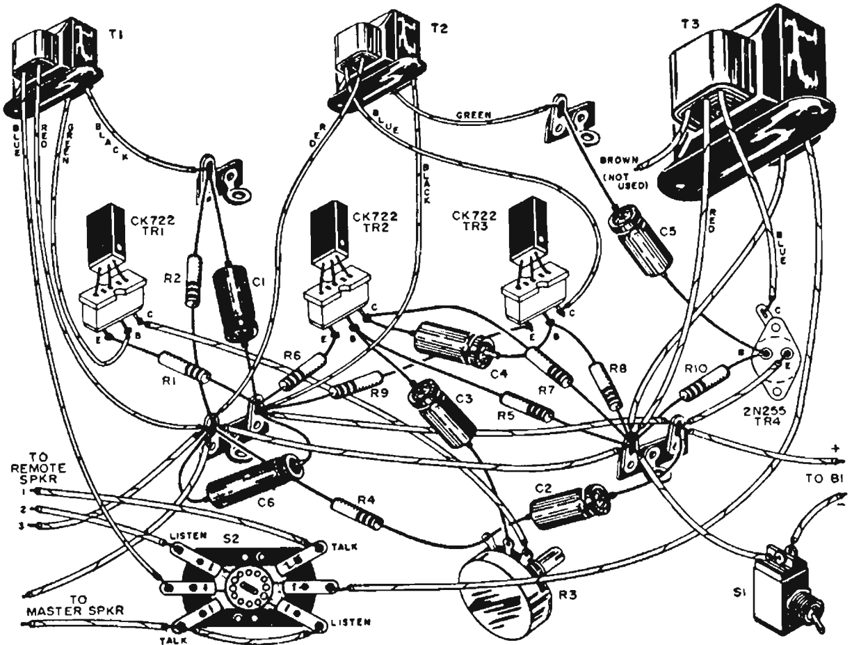
Fig. 162—Pictorial of parts mounting of transistor for final assembly.
