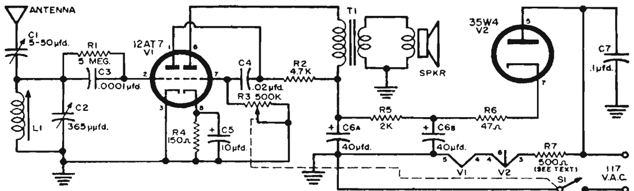
Fig. 137—Schematic for low-cost receiver. A 12AU7 can be used in place of the 12AT7 if it is easier to obtain.
