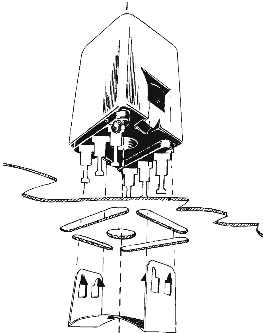
Fig. 37—Transformer mounting. Spring clip fits notches in side of can.
