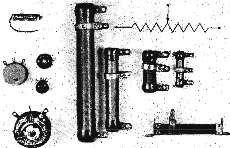
Fig. 31—Variable resistor types. Potentiometers are on the left; wire-wound types which have an adjustable tap are on the right.
