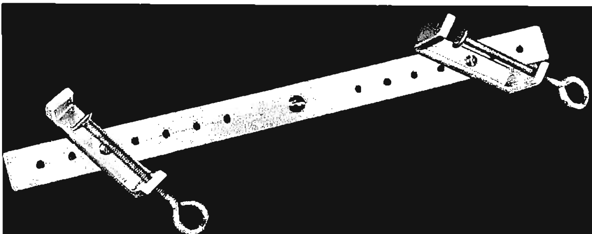
Fig. 92—Assembled rocker arm with clamps. Two of these arms are required.
