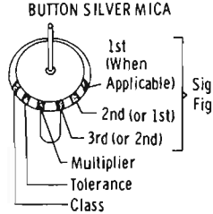
Fig. 33—Capacitor color code (continued).
