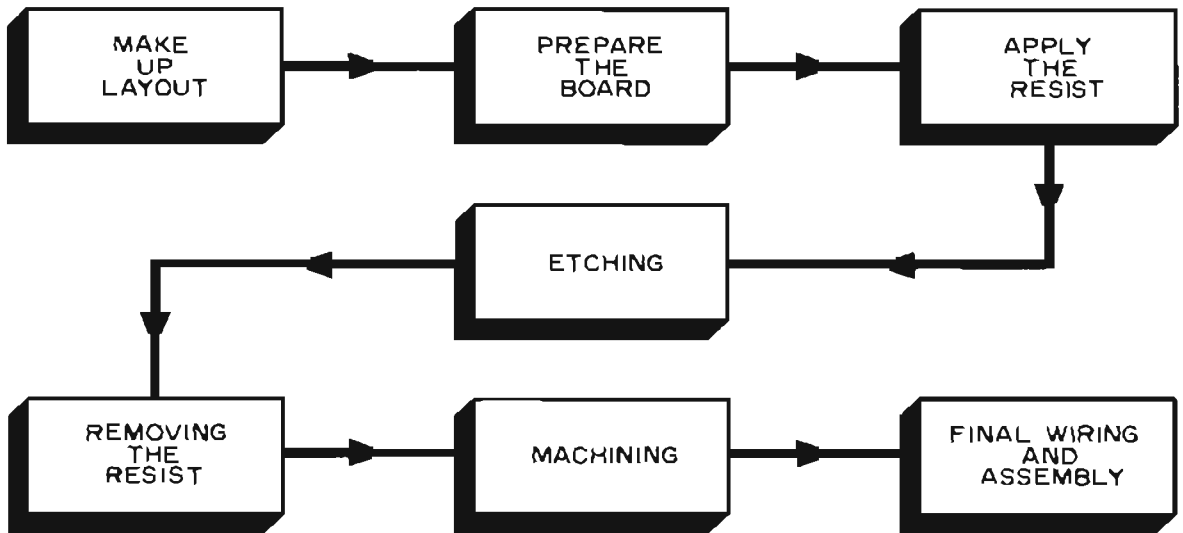
Fig. 56—Basic steps in the preparation of an etched circuit board.
