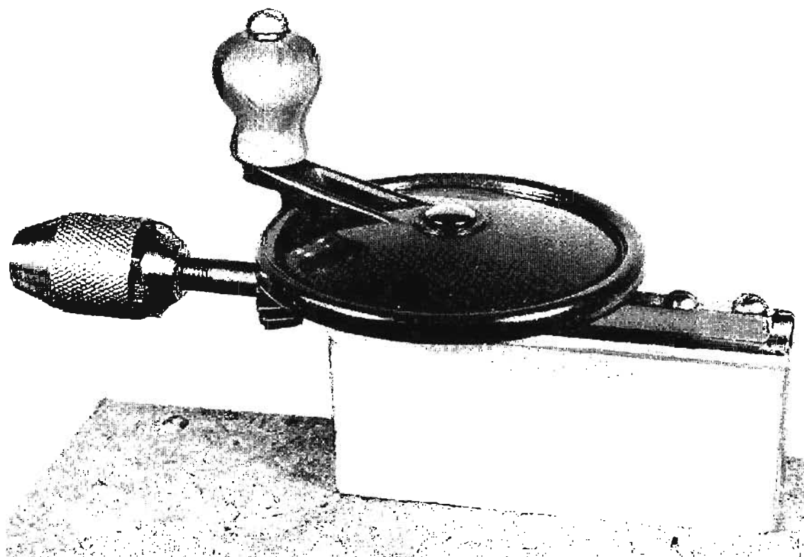
Fig. 102—Drill mechanism mounted on the base.
