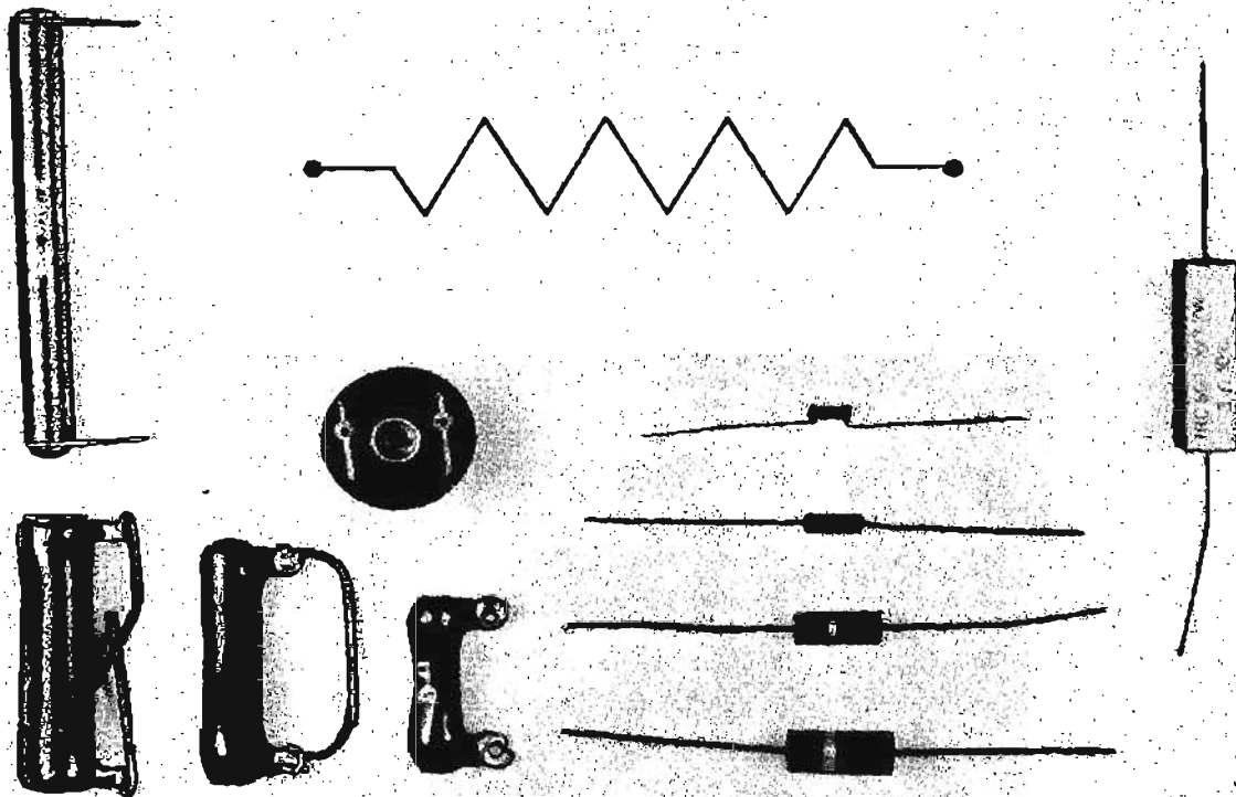
Fig. 29—Fixed resistors are indicated by symbol at top center. The units shown at left are wire wound; those at center are of a carbon composition. The rectangular unit at the right is a 7-watt resistor used in power-supply circuits.
