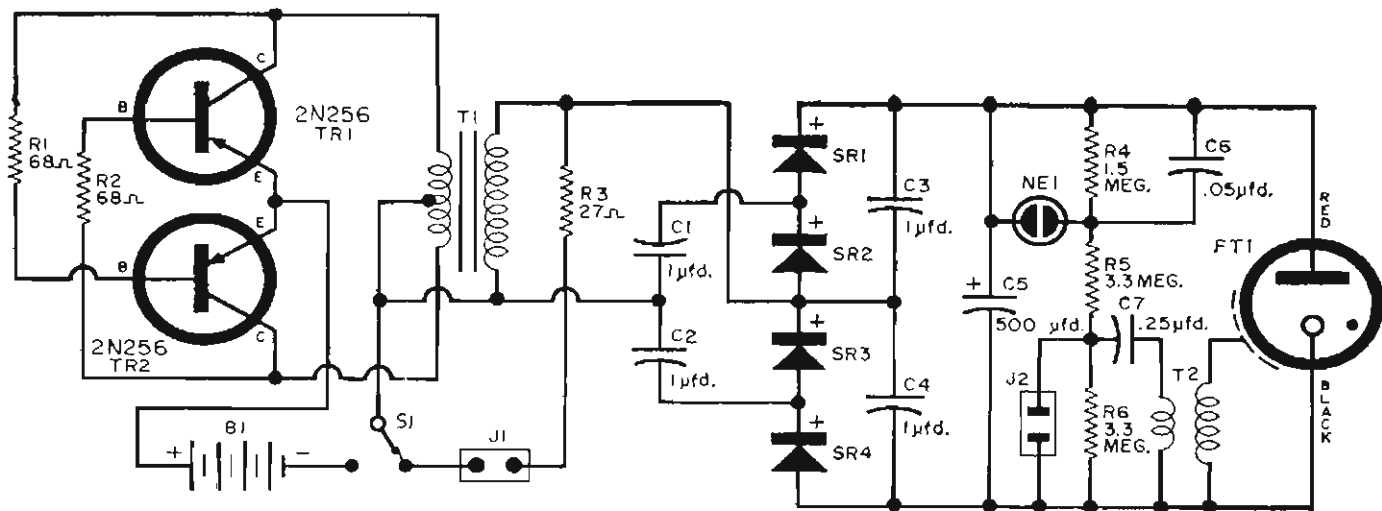
Fig. 168—Schematic of transistorized photoflash.
