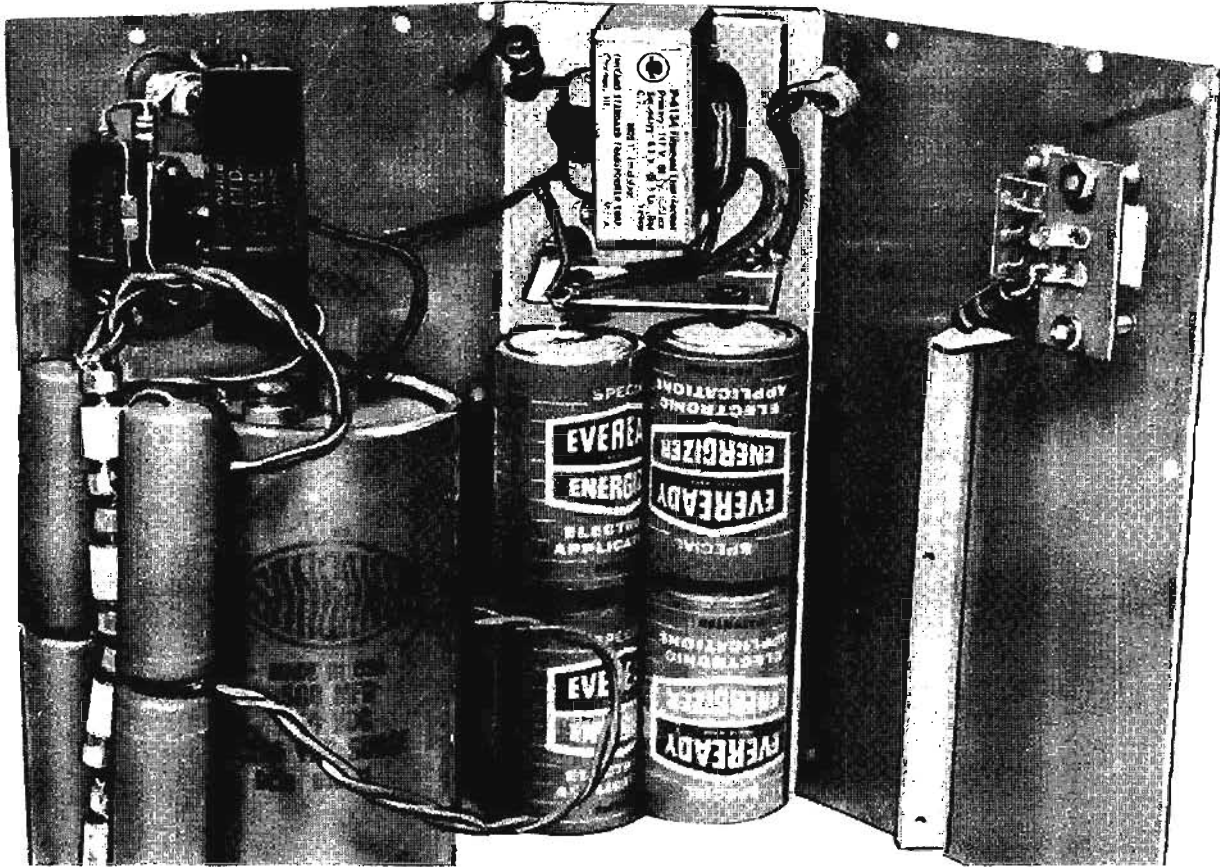
Fig. 169—Interior view of flash unit with front panel removed. Note the rods which hold the cells in place.
