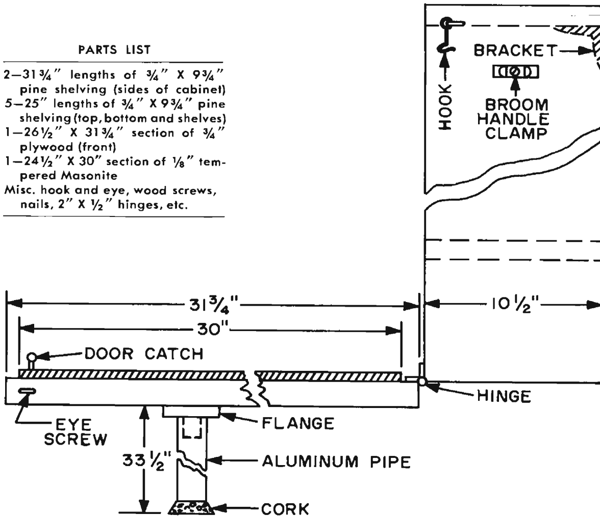
Fig. 68—Mechanical drawing of the "hidden" bench.
