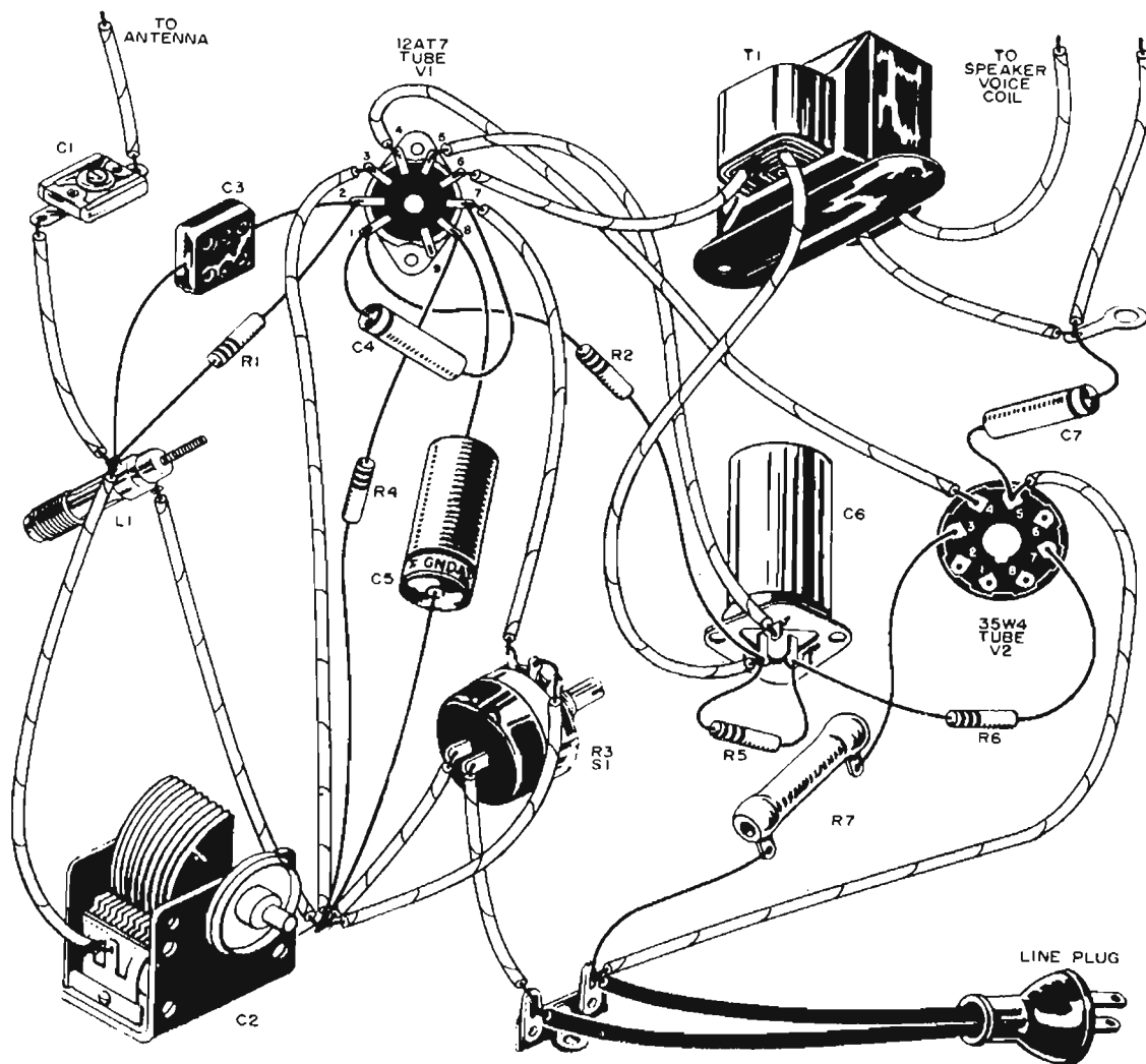
Fig. 138—Interconnect components as shown. Resistor R7 will get warm in normal operation.
