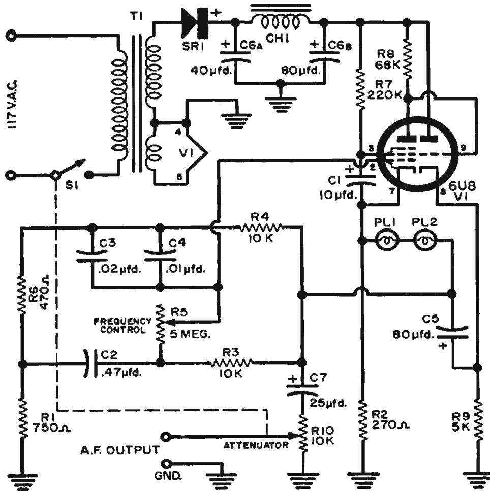
Fig. 126—Complete wiring details for audio oscillator.
