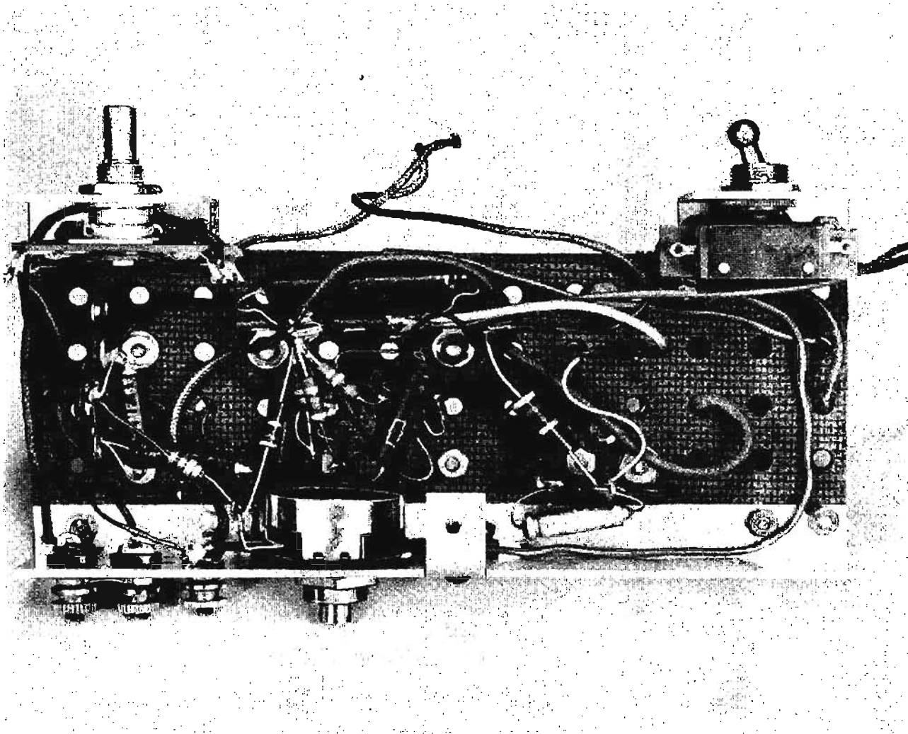
Fig. 163—Amplifier chassis shown from below with major parts installed.
