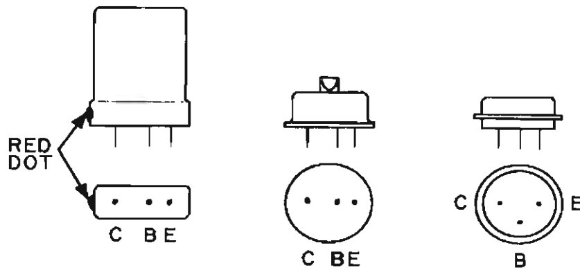
Fig. 26—Three placements of transistor leads.
