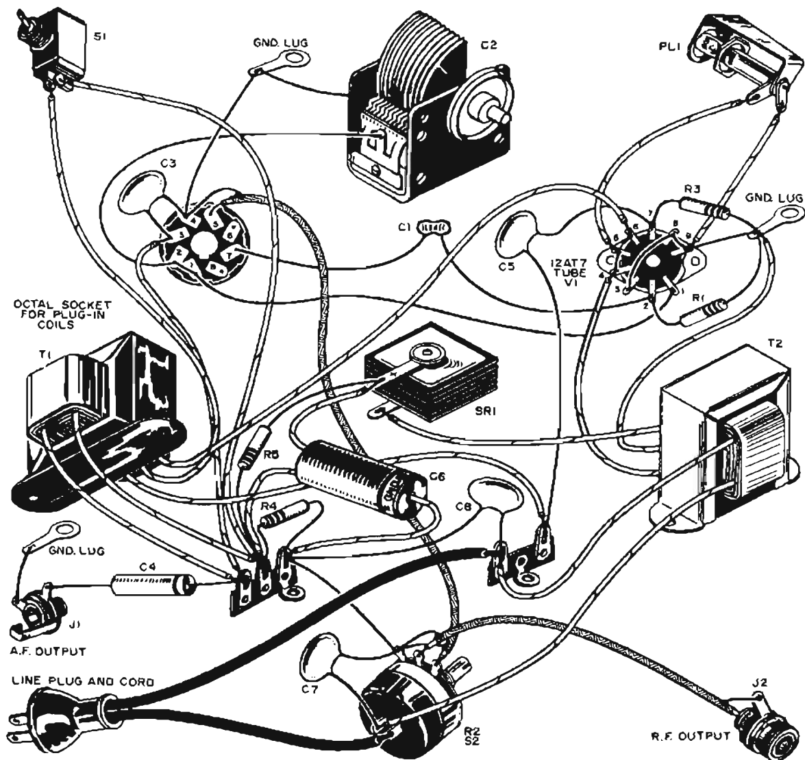
Fig. 130—Pictorial shows how parts of r-f signal generator are interconnected.
