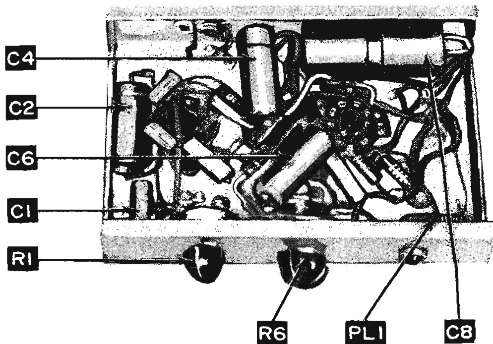
Fig. 125—View of audio generator. Note placement of major parts.
