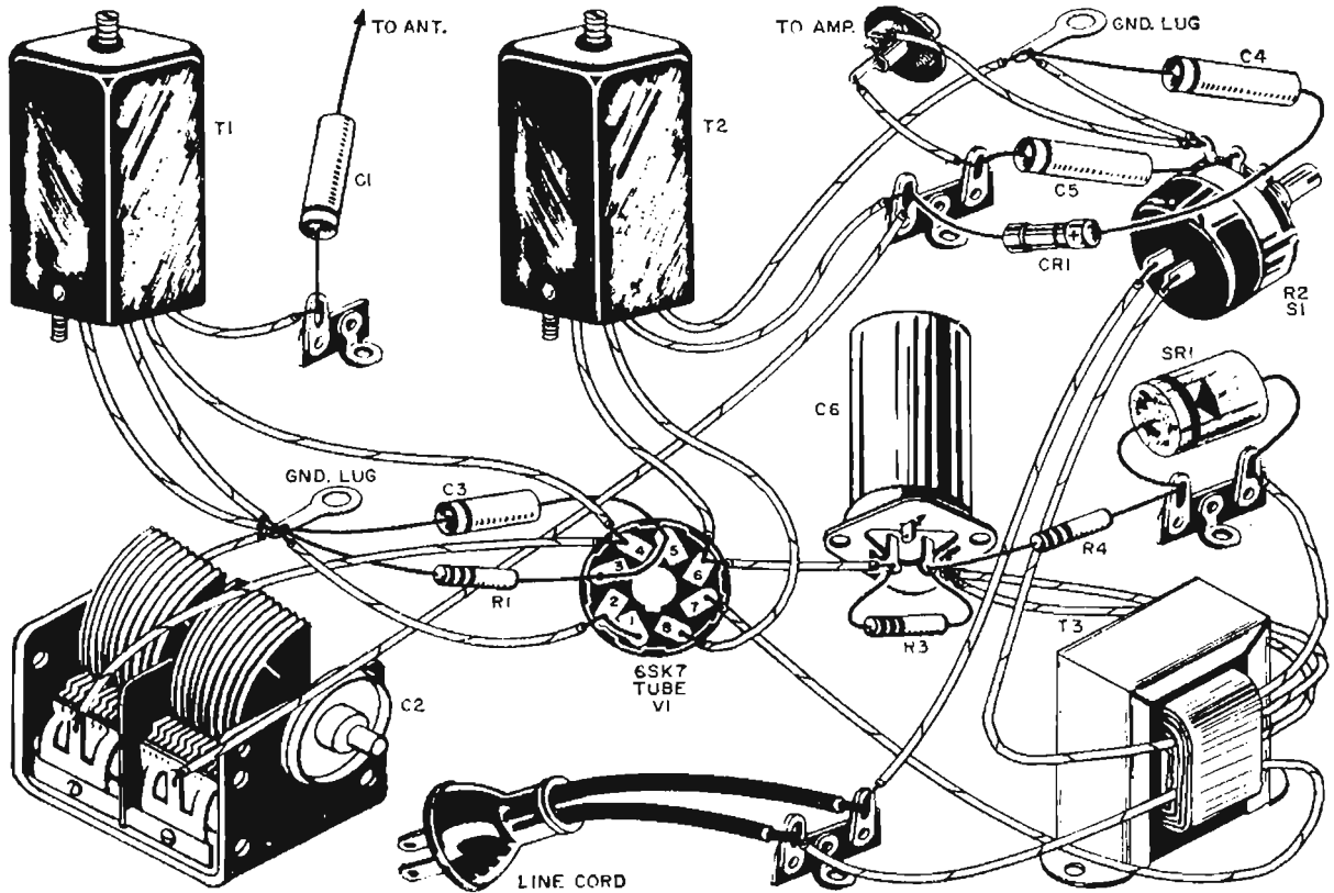
Fig. 142—Follow the pictorial diagram for best results in building the tuner.
