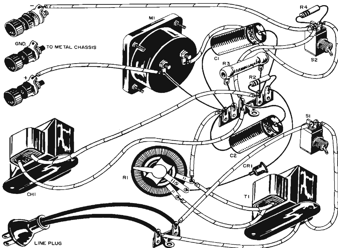
Fig. 123—Pictorial of power supply shows how parts are interconnected.
