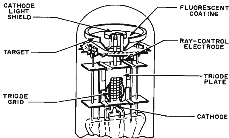
Fig. 22—Cross-section of a magic-eye tube.
