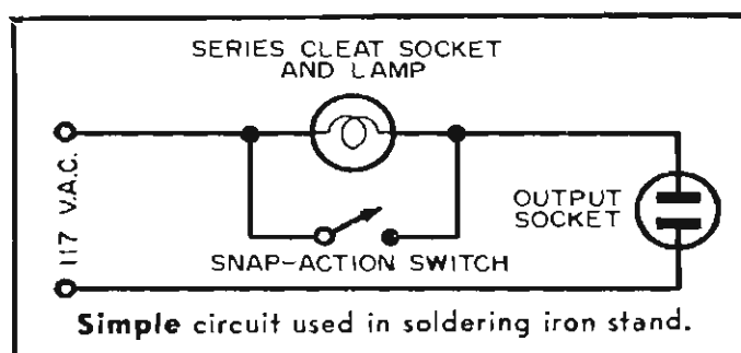
Fig. 77--Circuit for heat control unit.
