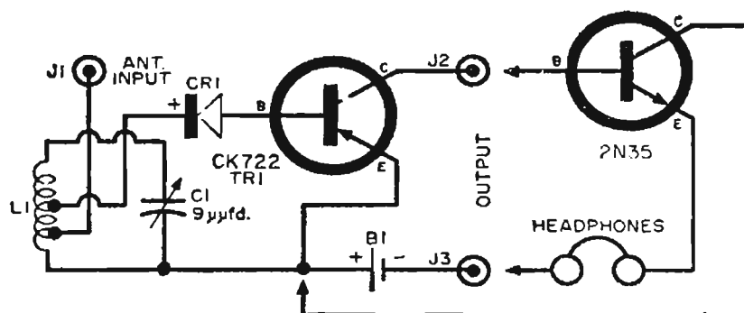
Fig. 154—Schematic diagram of receiver. Headphones can be plugged directly into output of single transistor, but greater volume results if transistor TR2 is added and J2/J3 repositioned in circuit.
