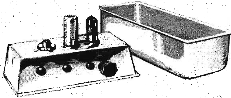
Fig. 48—Household pans used for chassis bases.
