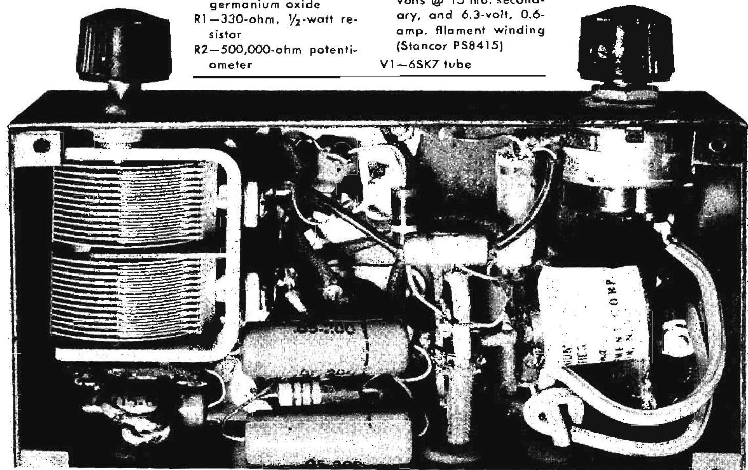
Fig. 140—Under-chassis view of the completed tuner shows parts placement.
