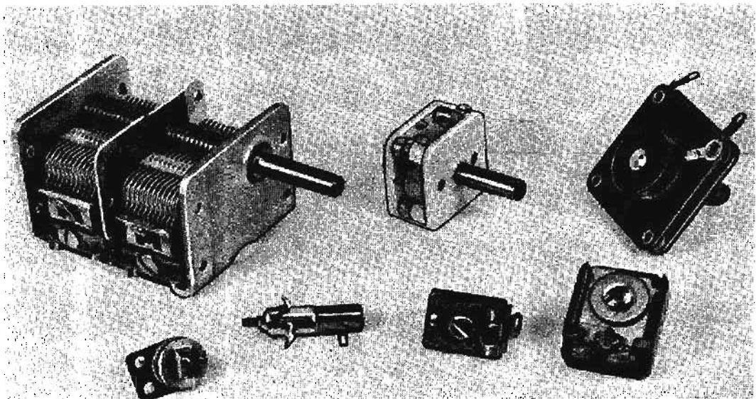
Fig. 34—Variable capacitors. Trimmer and padder types are at bottom.
