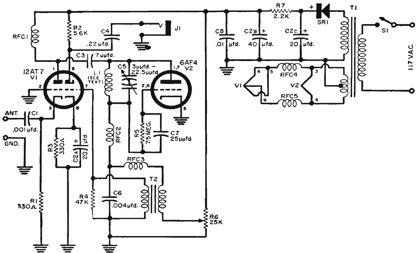
Fig. 147—Schematic for v.h.f. receiver.
