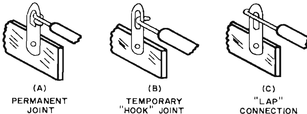
Fig. 15—Three types of mechanical connection used in soldering.
