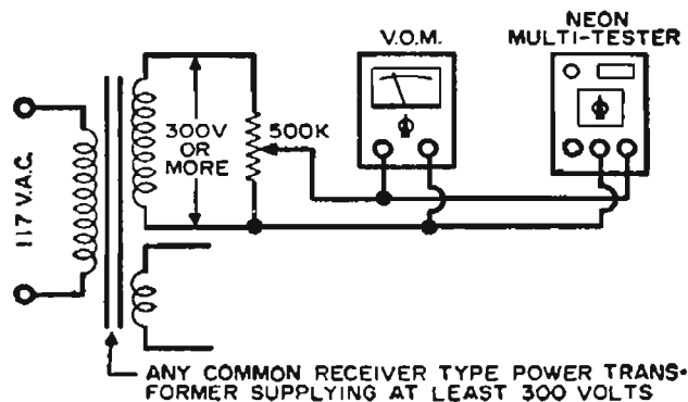
Fig. 112—Voltage calibrating setup for multi-meter.
