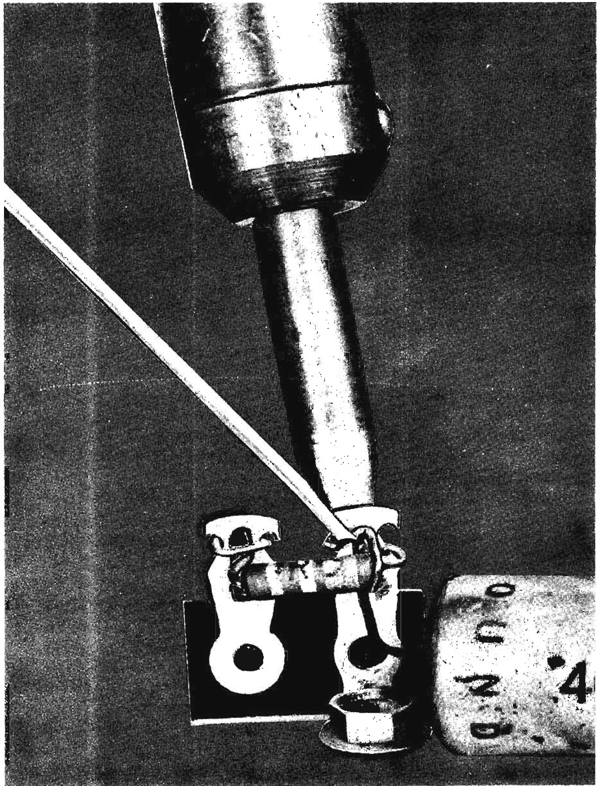
Fig. 4—Correct soldering technique.
