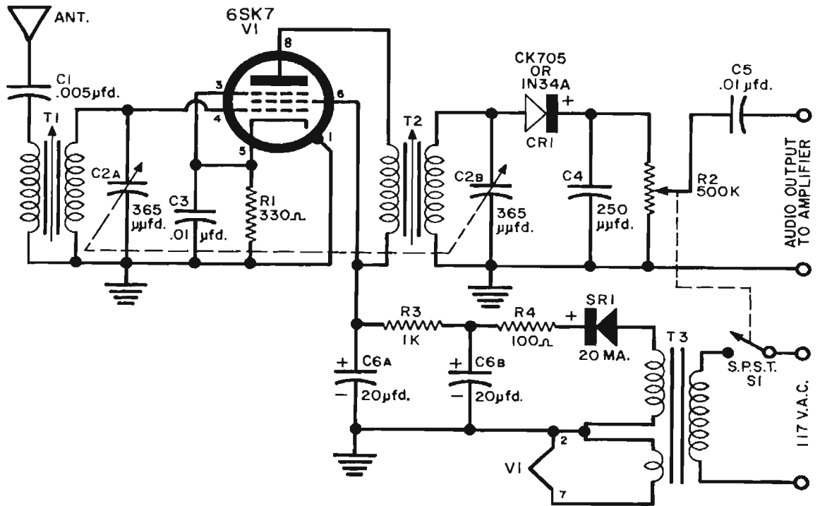
Fig. 141—Note the use of the power transformer to connect the tuner to any amplifier.
