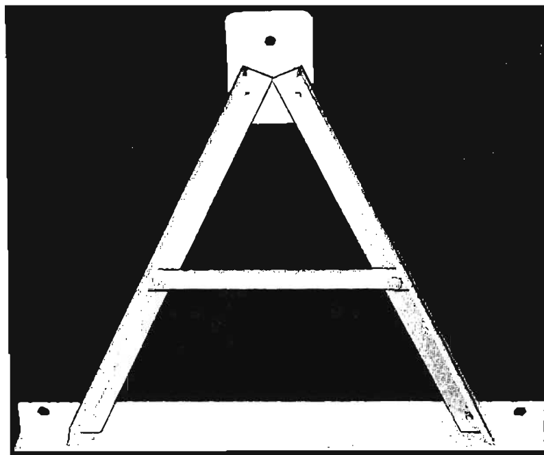
Fig. 90—Completely assembled A-frame.
