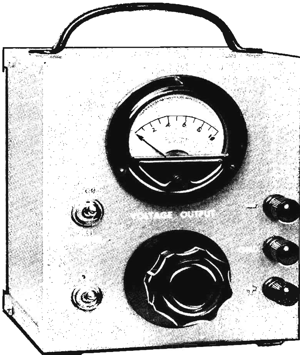
Fig. 121—Experimenter's transistor power supply.
