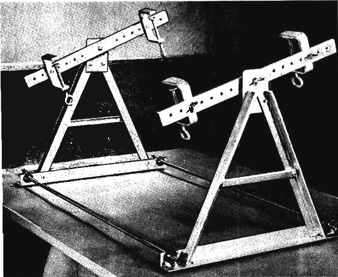
Fig. 95—Fully assembled chassis rack.
