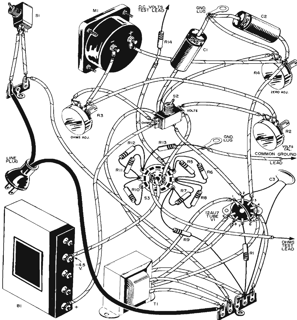
Fig. 114—Pictorial wiring diagram shows how various components are connected. Note particularly the wiring around switch S3 and shielded lead attached to R14.
