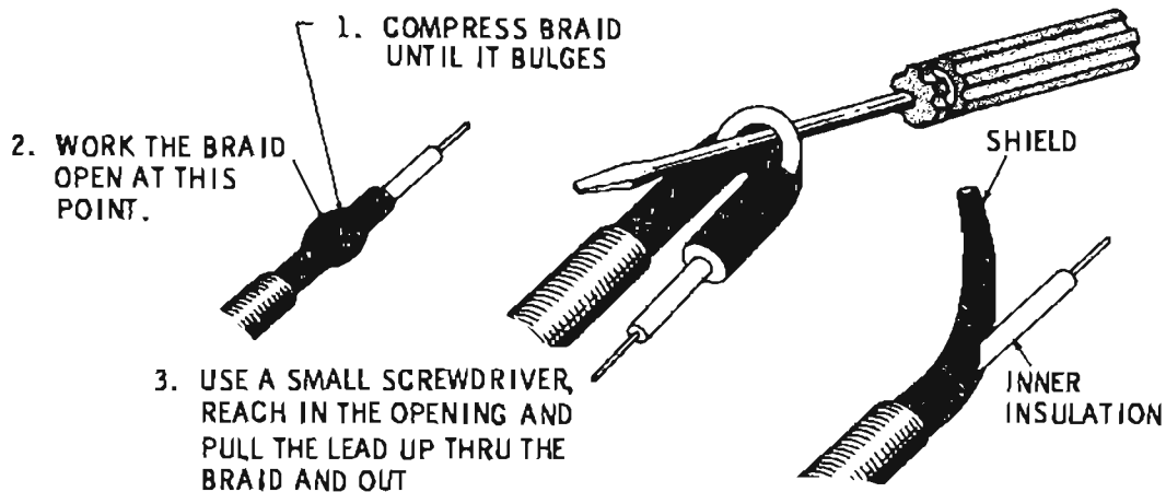
Fig. 16—Technique for stripping shielded cable.
