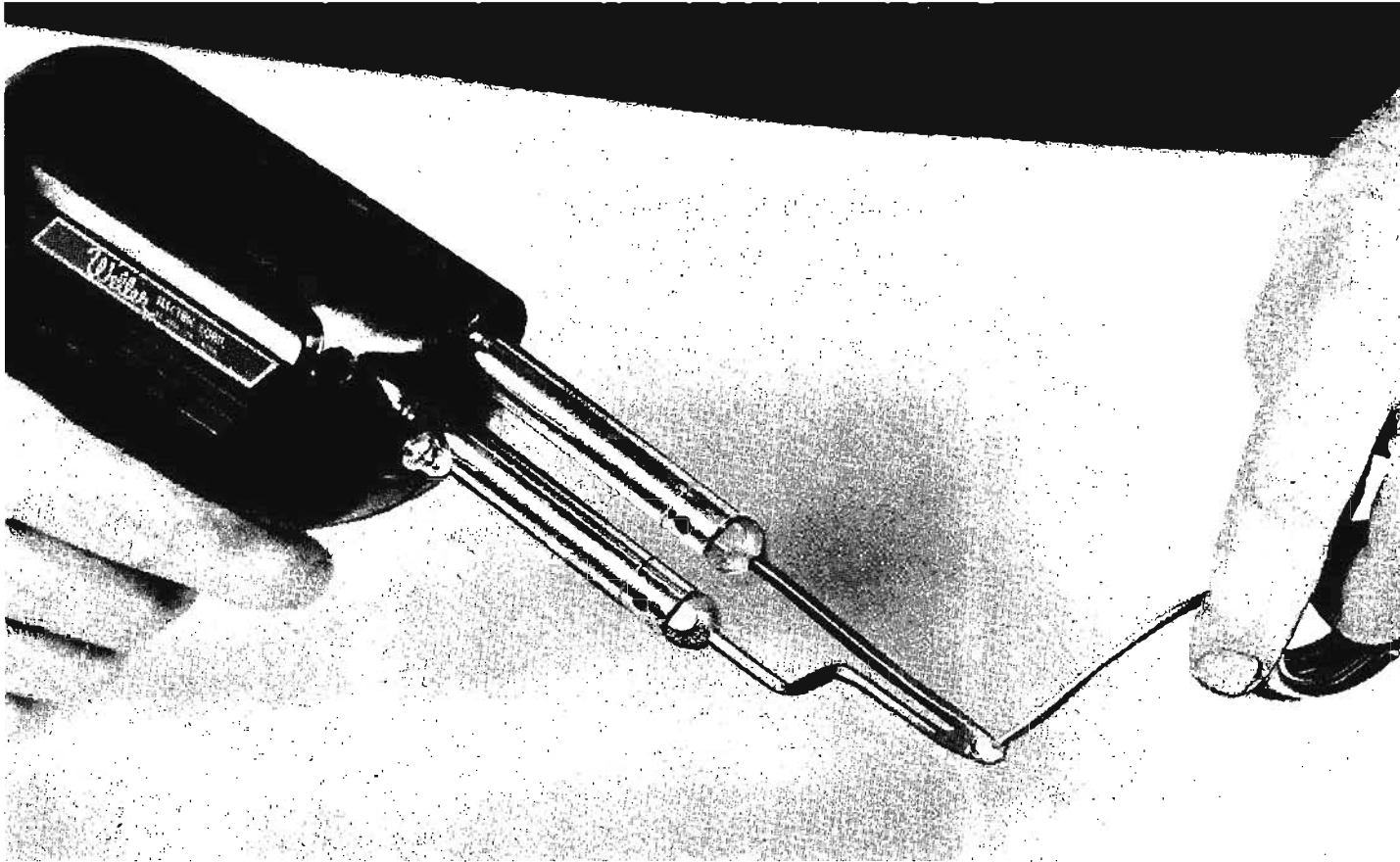
Fig. 5—Tinning the lip of a soldering gun.
