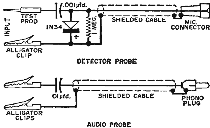
Fig. 136—These special probes should have all elements well shielded. The detector probe components can be built into a small tube shield. All capacitors should be 600-volt miniatures. Thin lapel microphone cable can be used for utmost flexibility.
