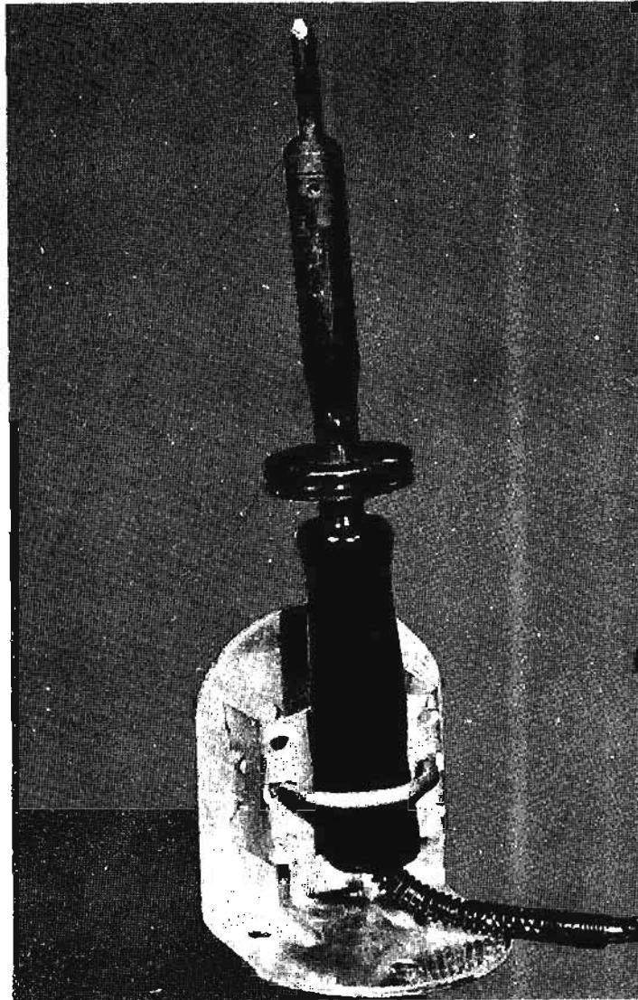
Fig. 78—A TV antenna mounting bracket used as a stand for soldering iron. Clamp can be tightened to attach it to the iron.
