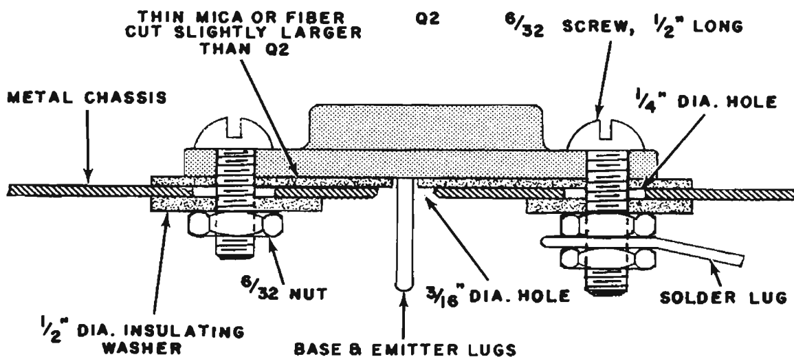
Fig. 27—Construction diagram of the mounting of a power transistor when the collector must be insulated from the chassis.
