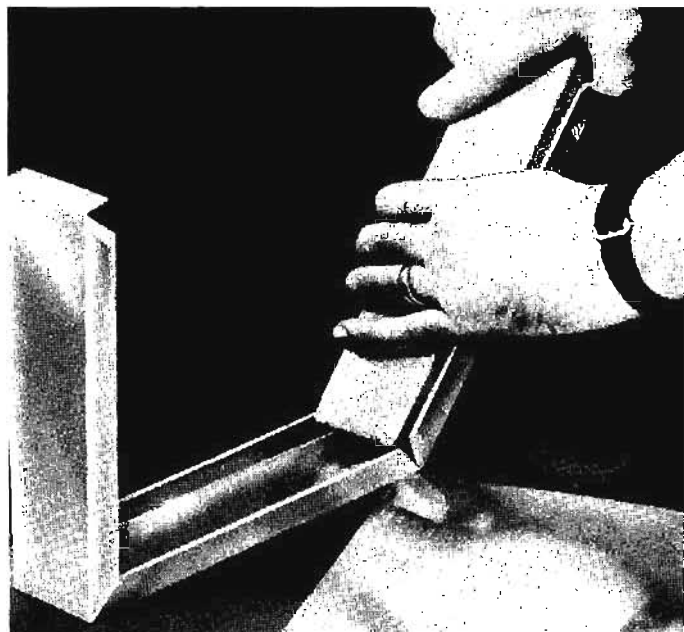
Fig. 46B—Bending aluminum with notches for desired chassis height.
