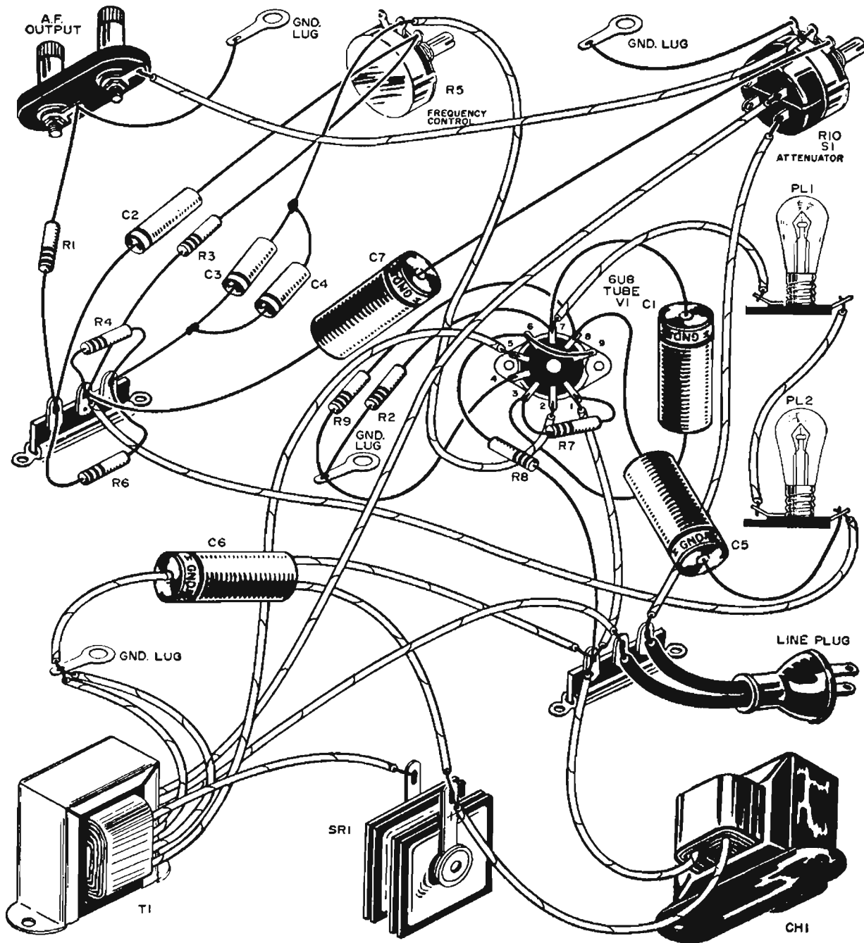
Fig. 127—Pictorial diagram of hook-up of audio-generator components.
