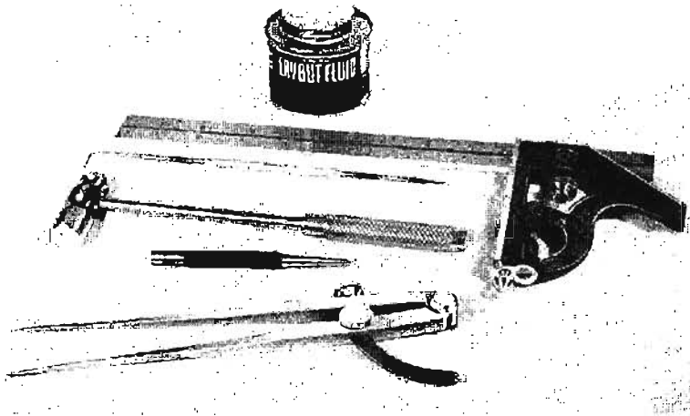
Fig. 42—Tools for chassis layout.
