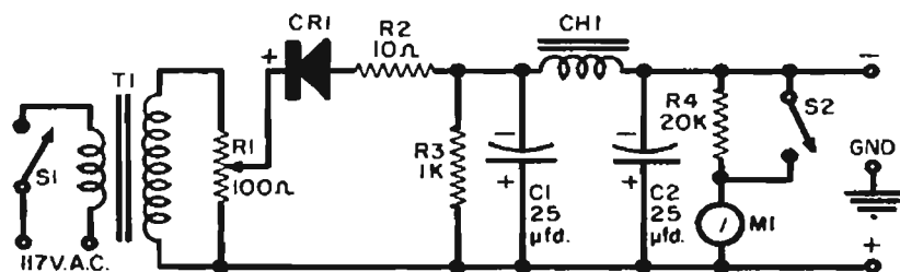
Fig. 122—Schematic diagram for transistor power supply.
