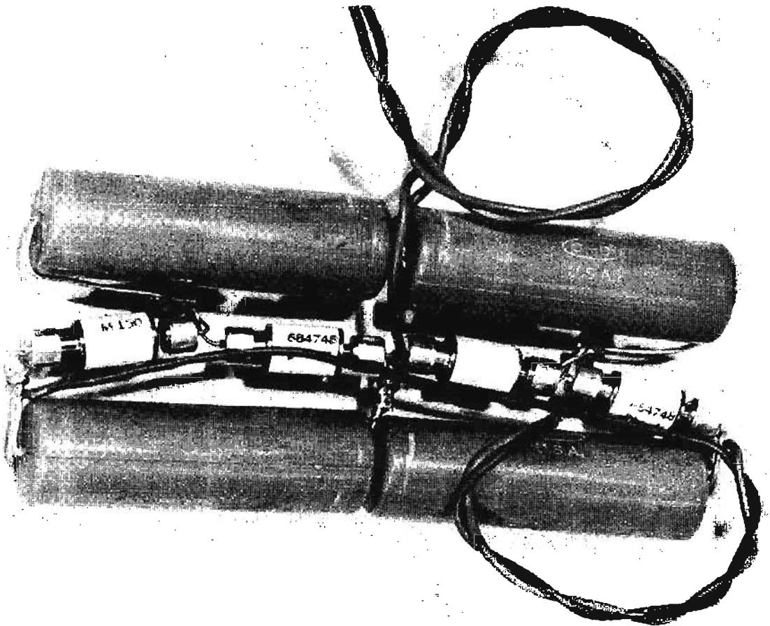
Fig. 170—Voltage quadrupler subassembly as it is wired immediately before being insulated.
