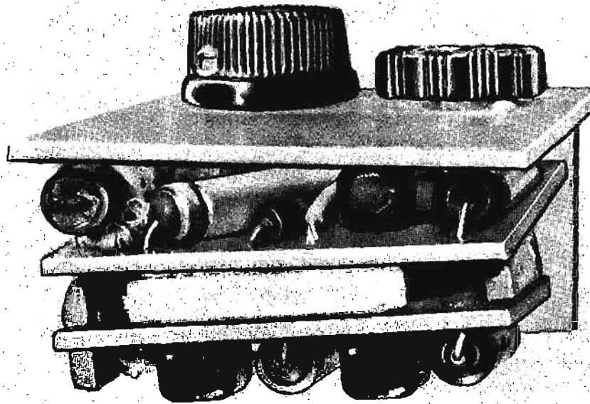
Fig. 150—Side view of the completed assembly. Note the small wooden spacers glued between the two printed-circuit chassis boards. The three sides and the bottom of the chassis are installed later.
