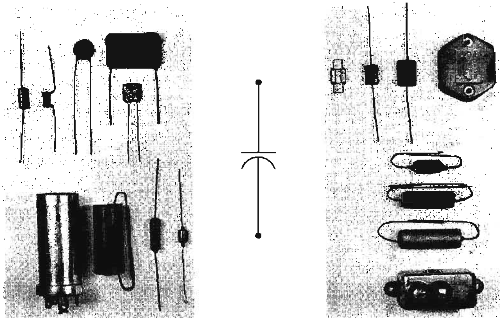
Fig. 32—Various shapes and sizes of fixed capacitors. Capacitor symbol is shown at center. Unit at lower left is can-type electrolytic.
