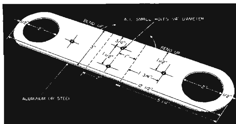
Fig. 83—Layout of the metal frame. The dimensions may be varied to suit the size of the clamp and solid rubber ball.
