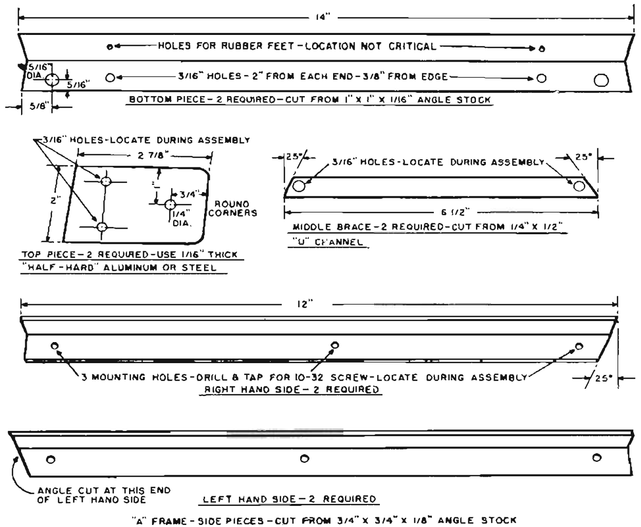
Fig. 89—Measurements of the pieces used to construct two A-frames.
