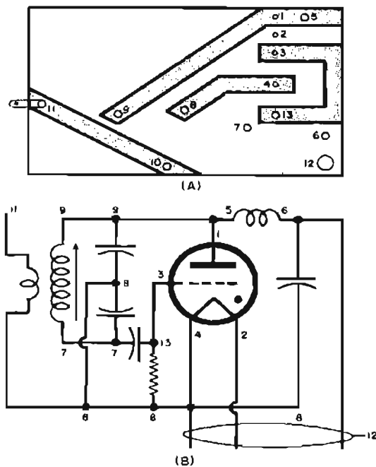
Fig. 63—Original radio control receiver circuit (top) and stripped circuit board (bottom). Numbers indicate corresponding points.
