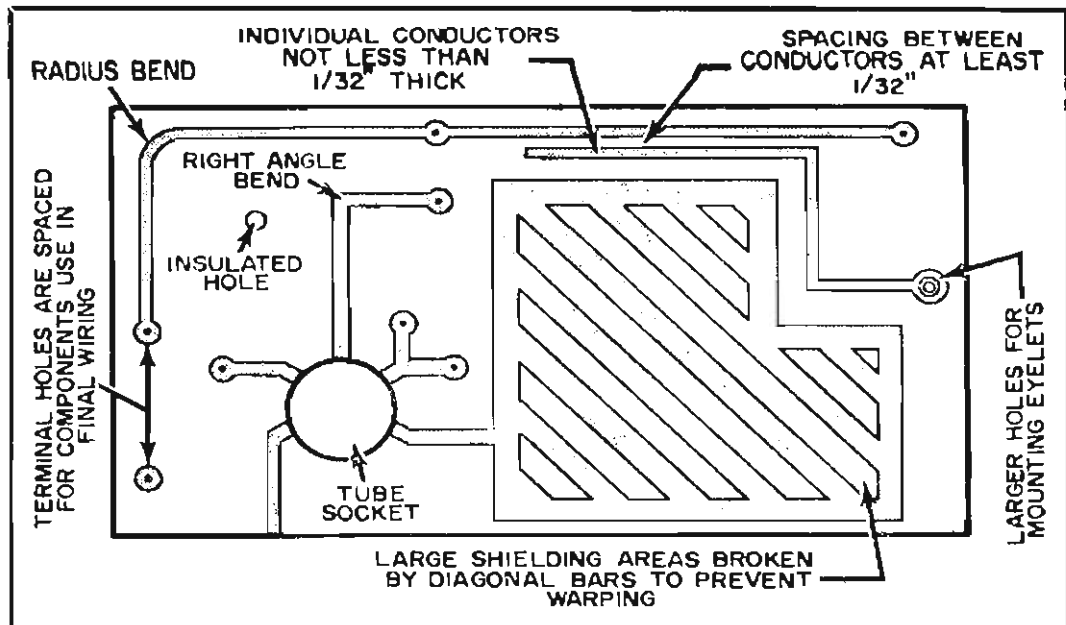
Fig. 59—Typical printed-circuit board.
