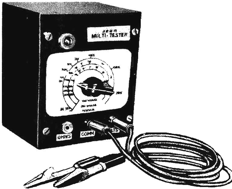
Fig. 110—Multi-tester with neon bulb which is used for economical construction.
