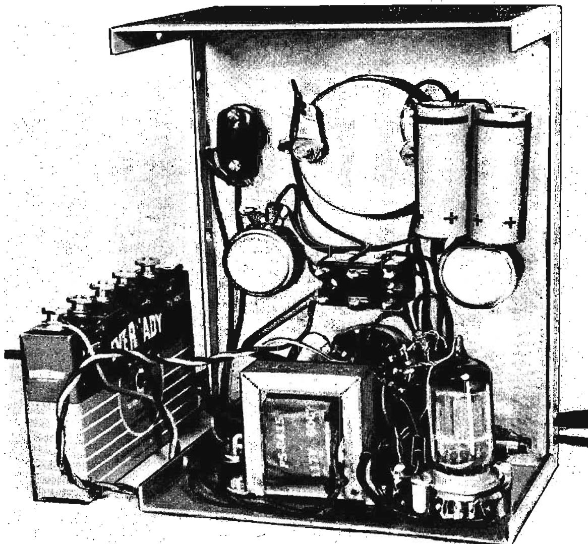
Fig. 116—Inside-the-case view of VTVM shows placement of parts used in original model.
