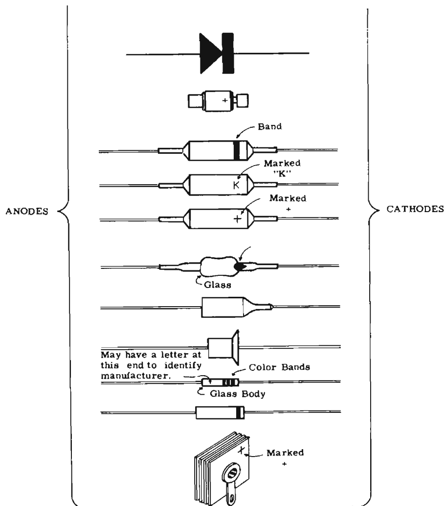
Fig. 28—Crystal diodes and rectifiers are marked in many ways. The symbol for all types shown here is at top.
