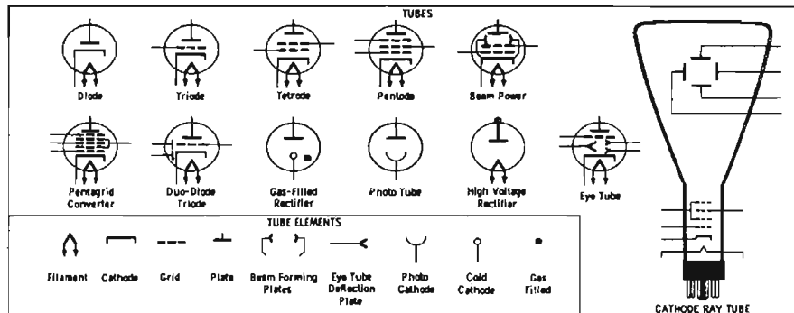
Fig. 21—Symbols for various tube types used by the experimenter.
