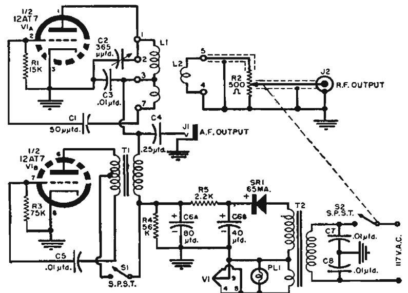
Fig. 129 — Circuit of radio-frequency signal generator.
