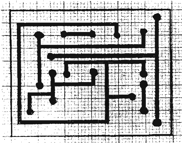
Fig. 58—Typical etched circuit layout.
