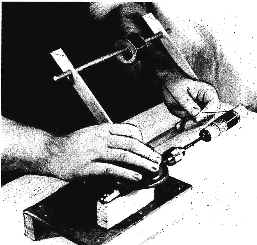
Fig. 100—Over-all view of the home-built coil-winding jig in operation. A "guide-paddle" is used to ensure level winding and professional appearance.
