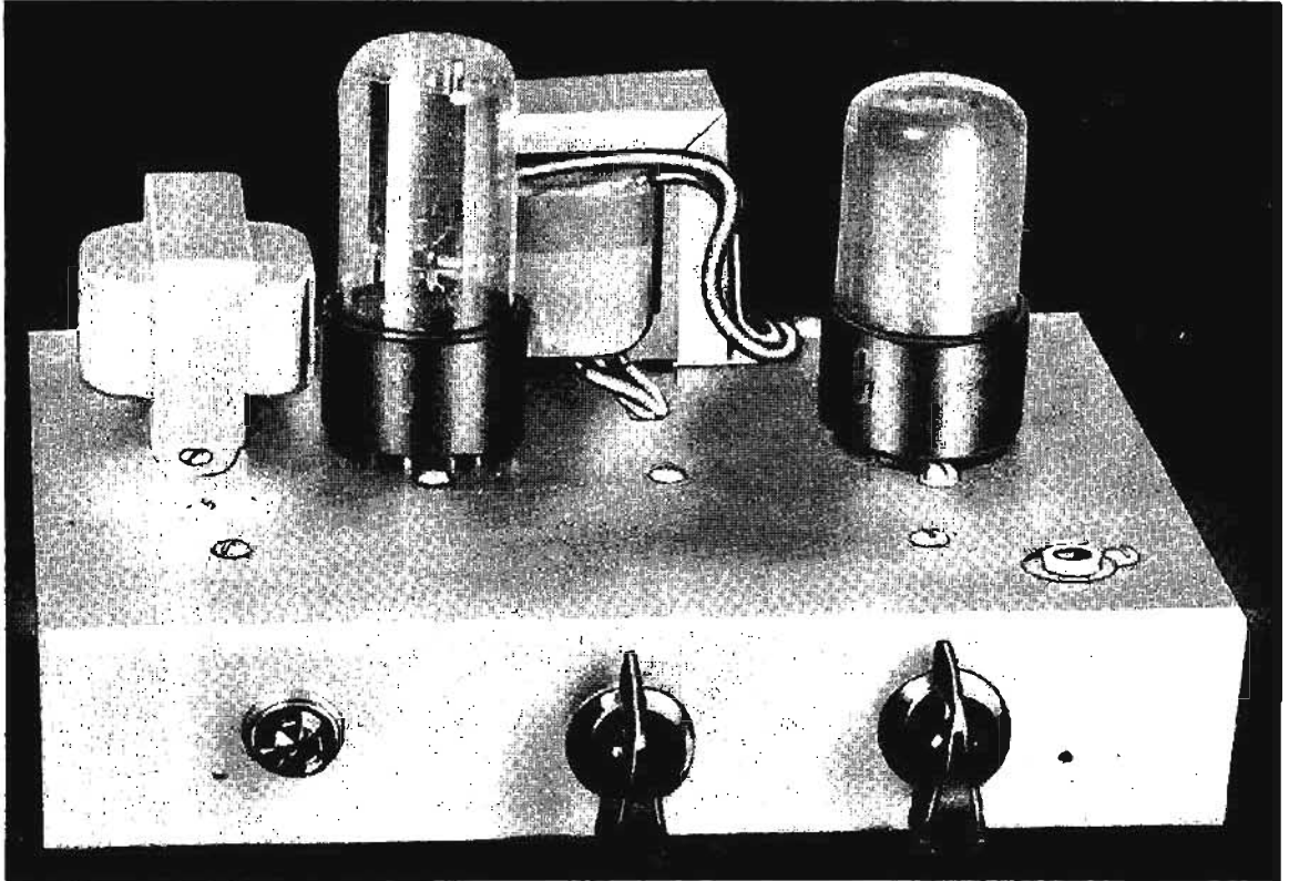
Fig. 156—Two-tube power amplifier. Pilot light, tone control, and volume control are on front panel.
