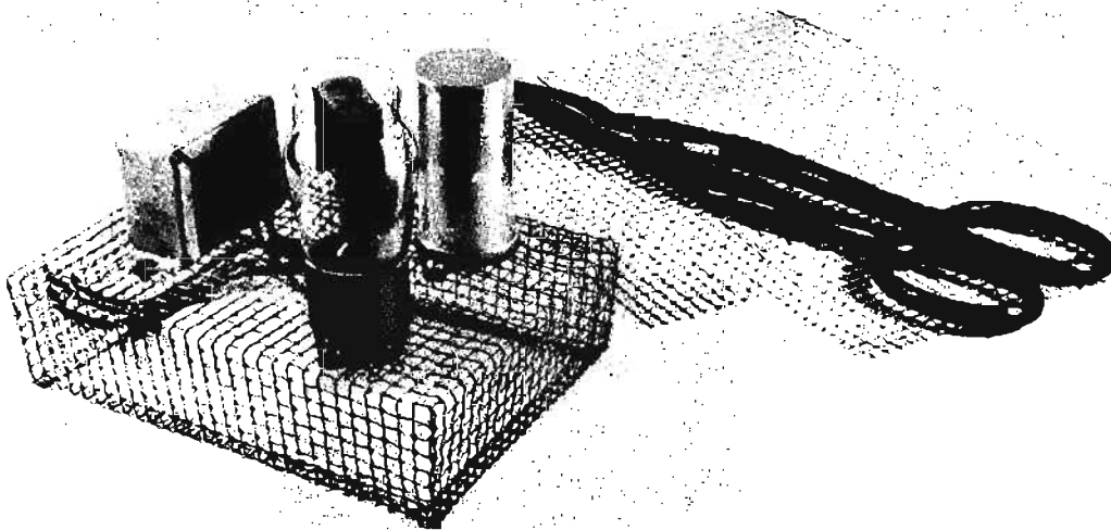
Fig. 49—Hardware cloth cut with metal shears and shaped to form a chassis. Corners are held together by soldering or by wrapping ends of wire mesh together.
