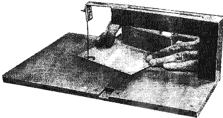
Fig. 96—How to use the completed plastic cutter to make right angles on \frac{1}{16} -inch Lucite.
