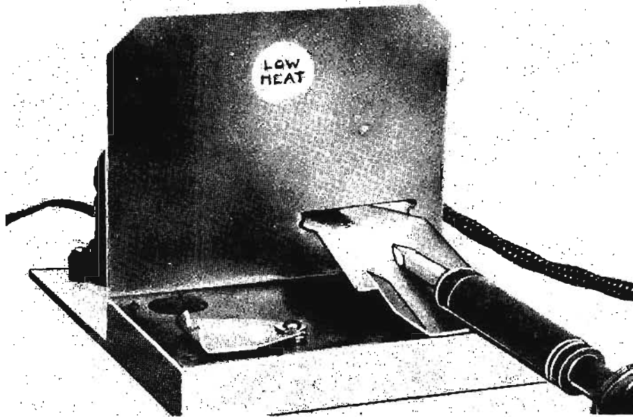
Fig. 75—Vertical section is aluminum; it is bent where it joins base block. Slit in lower right corner accommodates rocker-arm rest. Two circular holes must be punched in aluminum to match holes for cleaner and rosin cups in base block.
