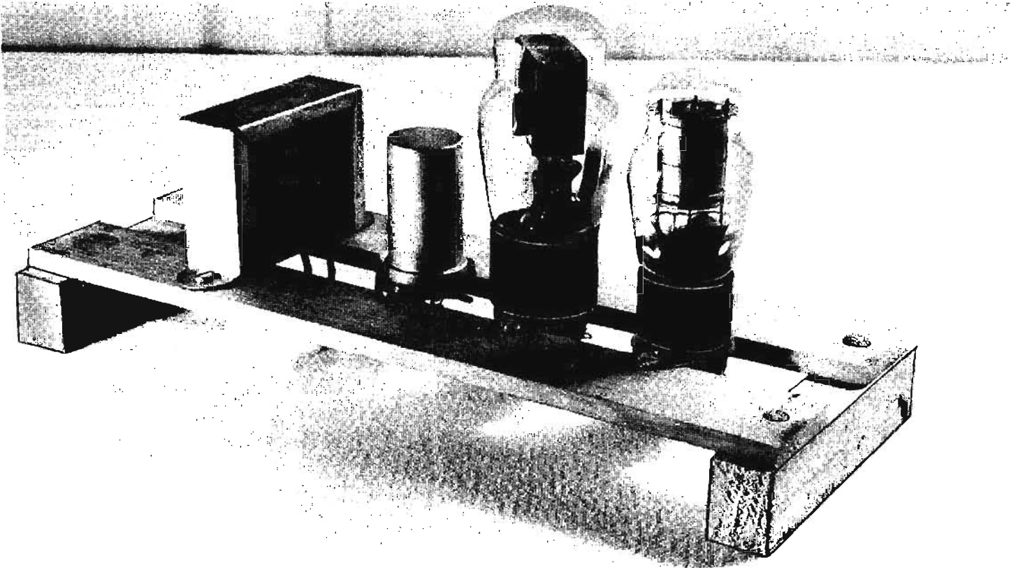
Fig. 51—Scraps of wood used to make a chassis base.
