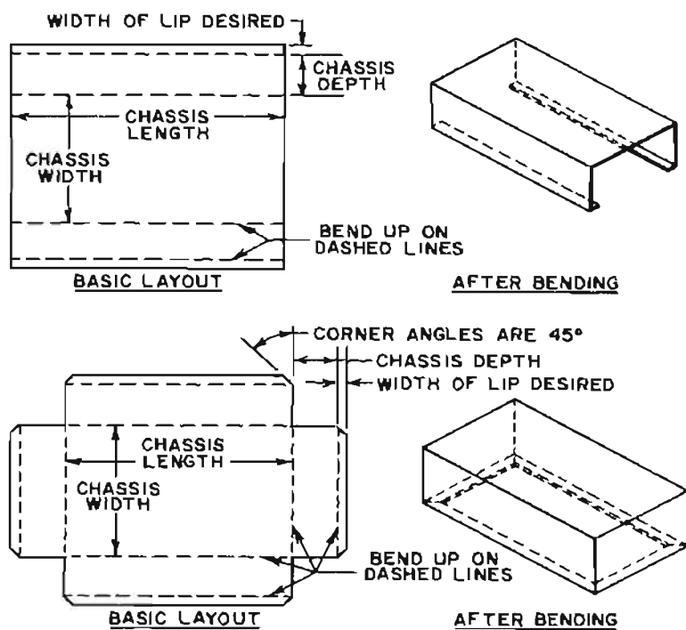
Fig. 47—Alternative chassis arrangements. Upper shows layout for chamele-type chassis. Lower shows box-type layout.
