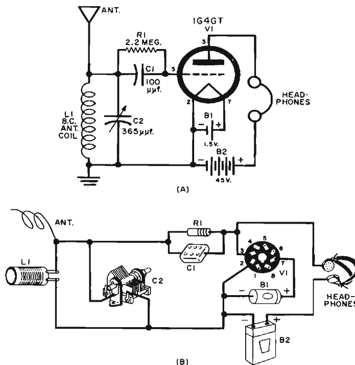
Fig. 55—Schematic for a simple radio.
