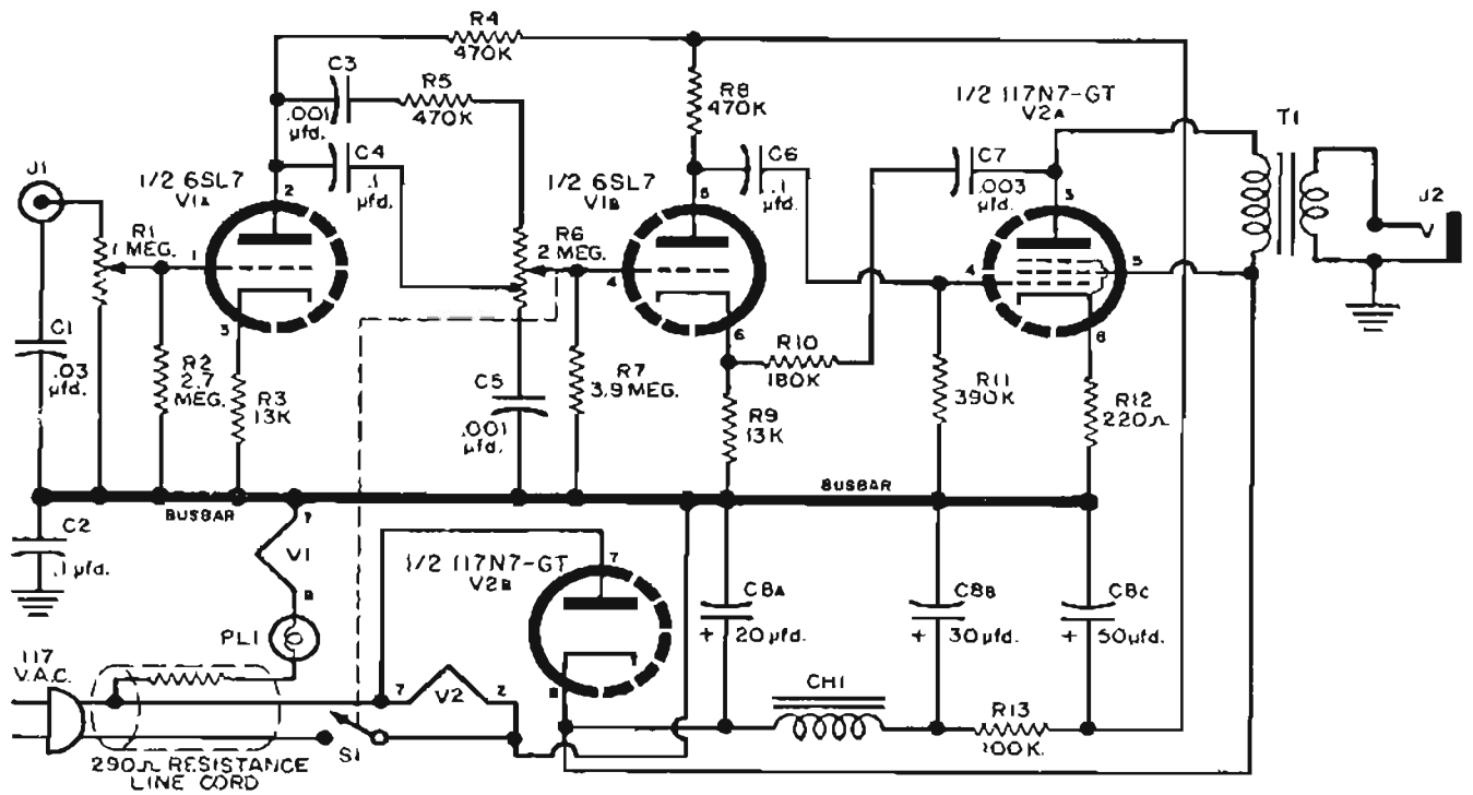
Fig. 157—Schematic of two-tube amplifier.
