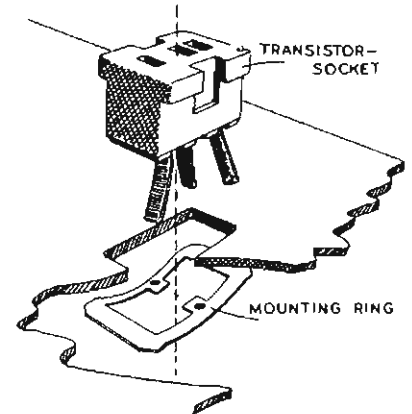
Fig. 25—Transistor socket mounted on a chassis by a metal clip that fits grooves in side of socket.
