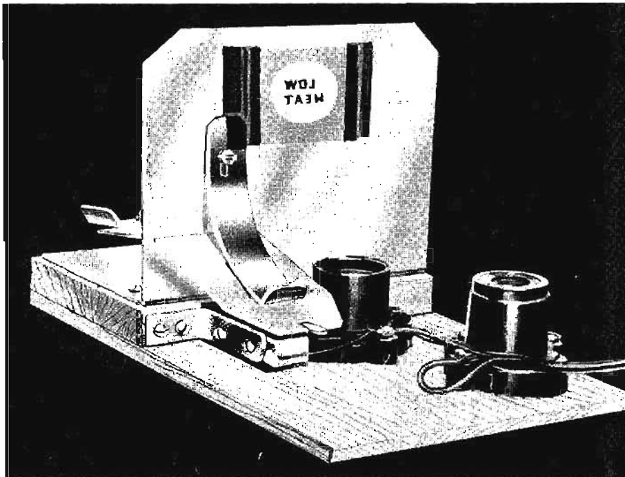
Fig. 76—Close-up of completed stand from opposite side. The socket in the foreground is used to plug in the iron, the other—near rocker—holds a 100-watt bulb.
