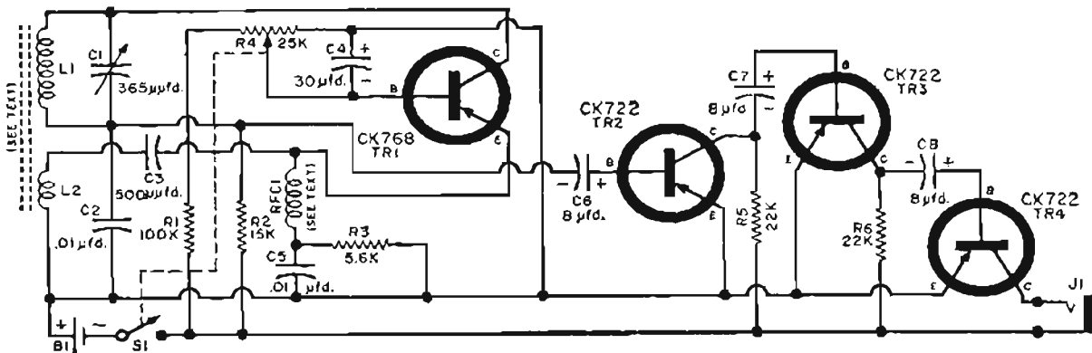
Fig. 152—Schematic diagram of transistorized receiver.
